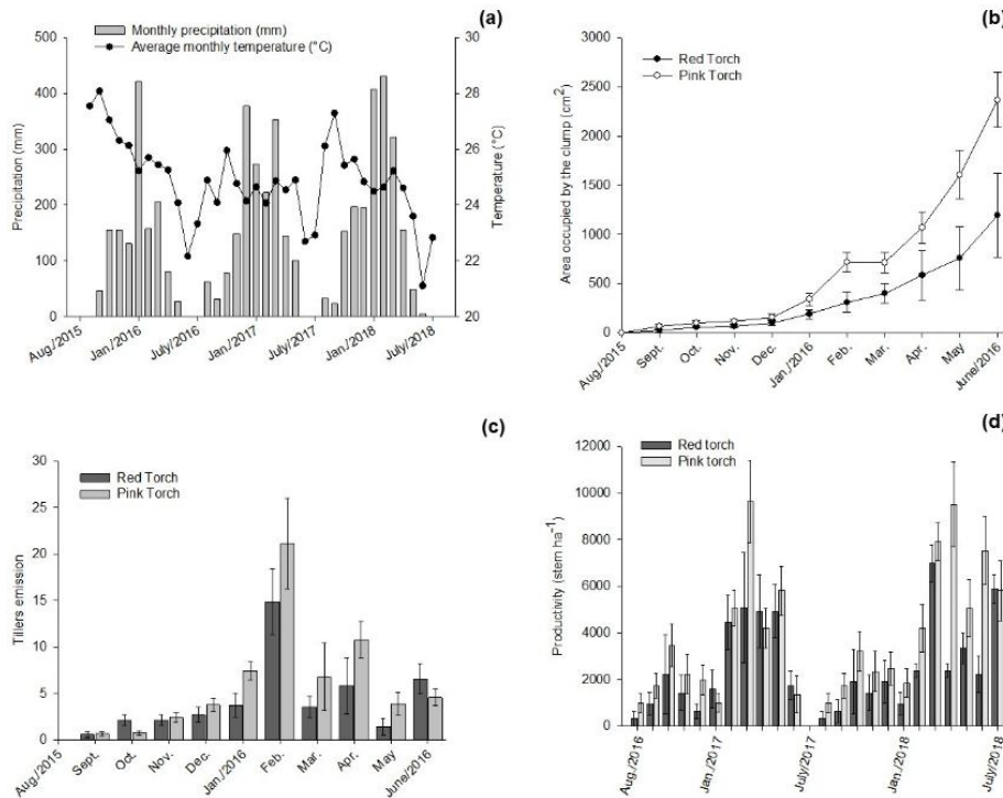
Fig. 2. Monthly precipitation and average temperatures from August 2015 to July 2018 (a); area occupied by torch ginger clumps (b); monthly emergence of tillers from clumps in the first year of cultivation (c); and productivity during the period from August 2016 to July 2018 (d). Error bars indicate standard errors. Tangará da Serra (MT), Brazil
