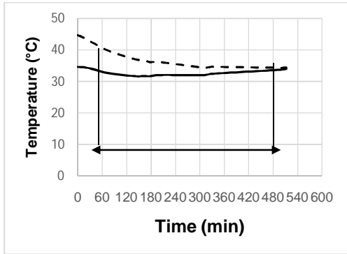
Figure 3: Temperature profile in fridge (solid line: fridge; broken line food) (a) and thermos flask (solid line: thermos flask; broken line food) (b) during conservation.
