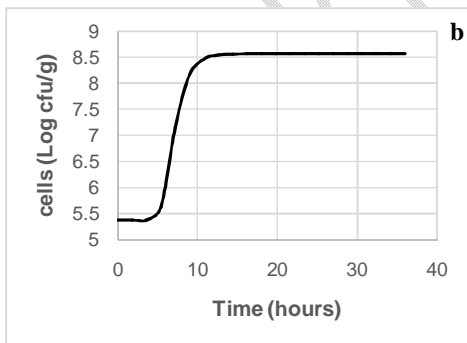
Figure 4: Outgrowth kinetic of Bacillus cereus spores in fridge (broken line) (a) and thermos flask (solid line) (b) during conservation
