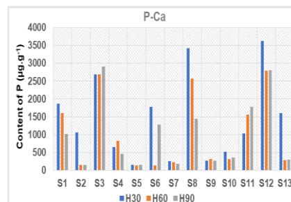
Figure 11: Phosphorus bound to calcium
