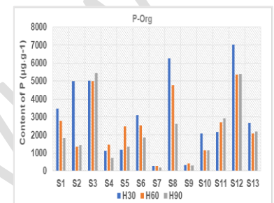
Figure 12: Phosphorus bound to Organic
