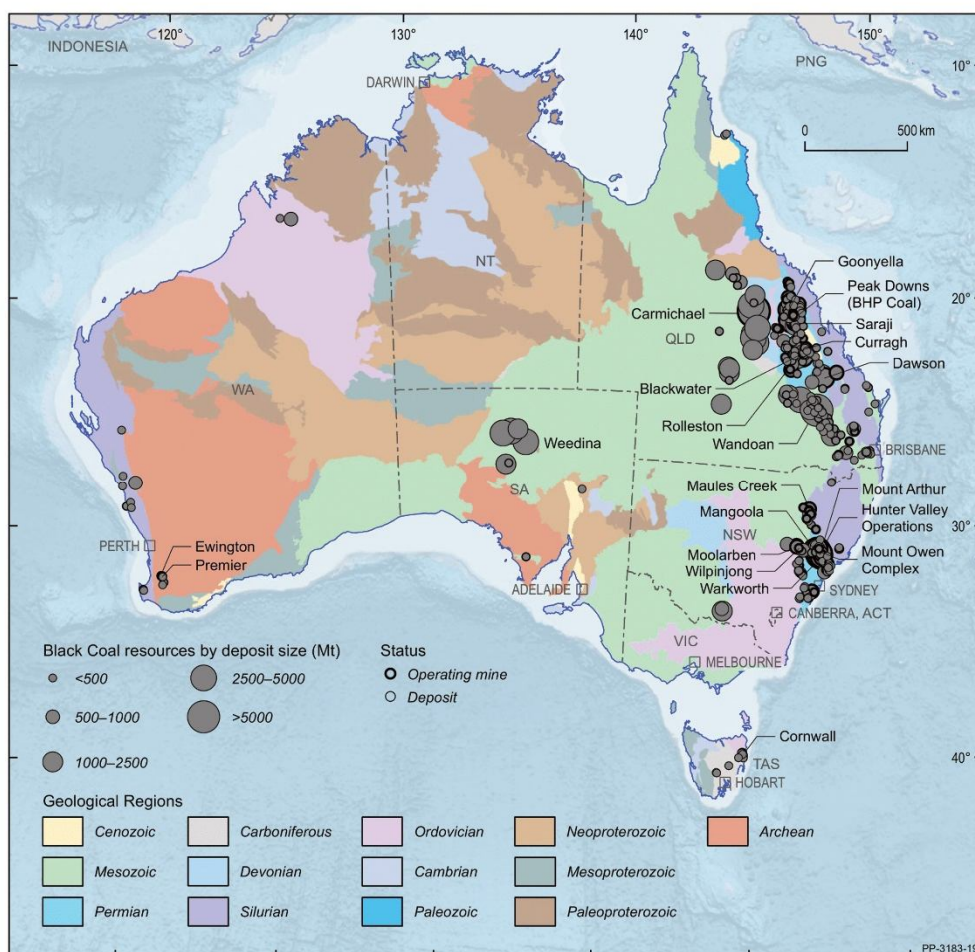
Figure 4. Black coal deposits and operating mines in Australia, 2018. (Aussie Maps – reddit.com)
