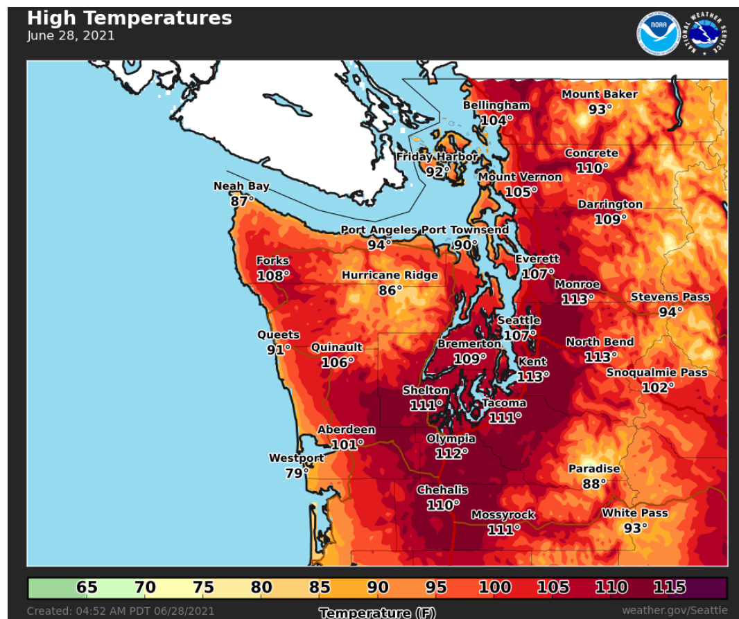
Figure 3. Washington state map of temperature on June 28, 2021. (NOAA)
