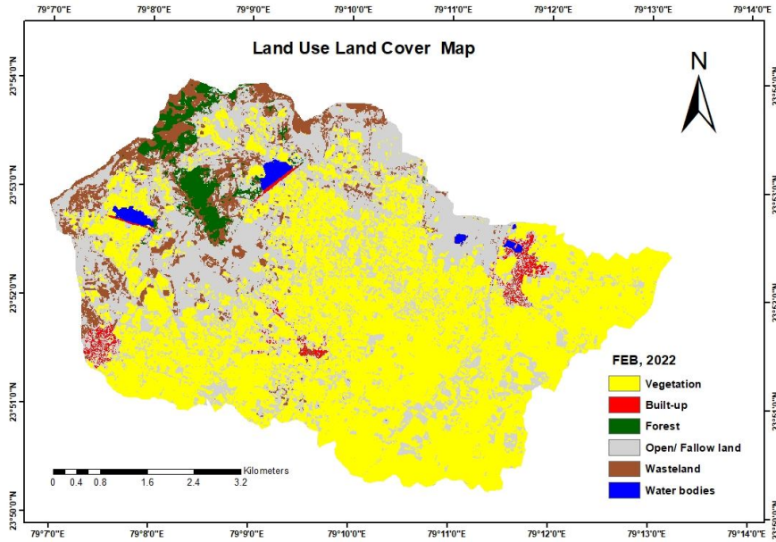
Fig 2: Land Use Land Cover Map for February,2022
