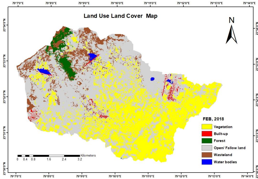
Fig 1: Land Use Land Cover Map for February, 2018
