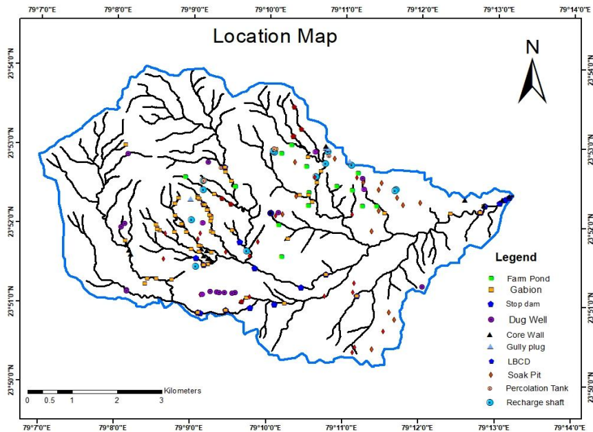
Fig. 3: Structure location and Stream order map
