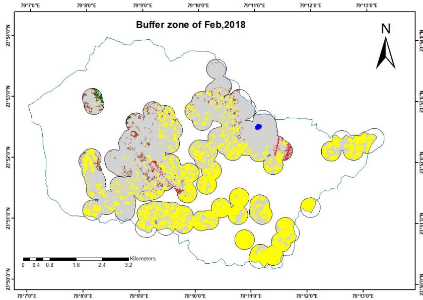
Fig 4: Buffer zone for February, 2018
