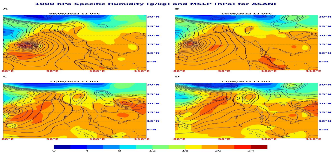
Fig:5 1000hpa specific humidity (g/Kg) and MSLP in hpa.
