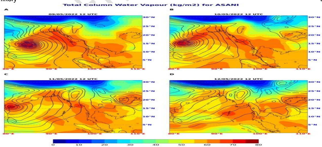
Figure 4 shows the total column water vapour (Kg/m2).
