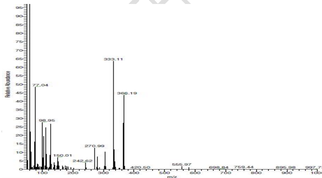
Fig(6) Mass spectrum of [Co(HL1) 2 ]
