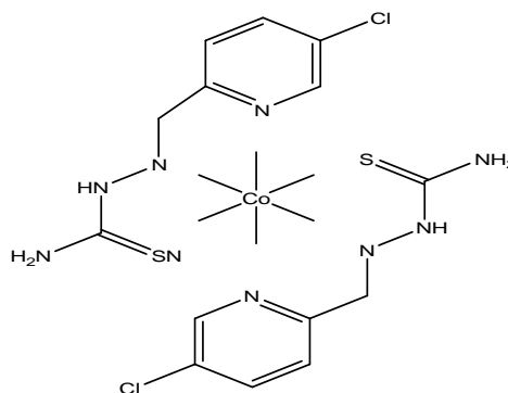
Fig (10): The probable structure of complex [Co (HL1) 2 ]
