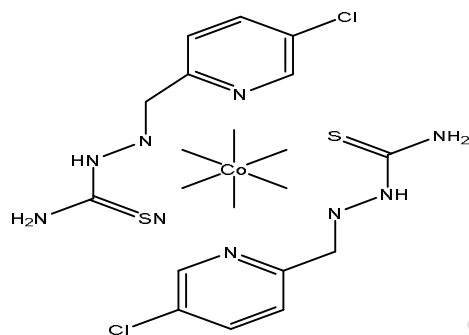
Fig (11): The probable structure of complex [Ni (HL1)2]
