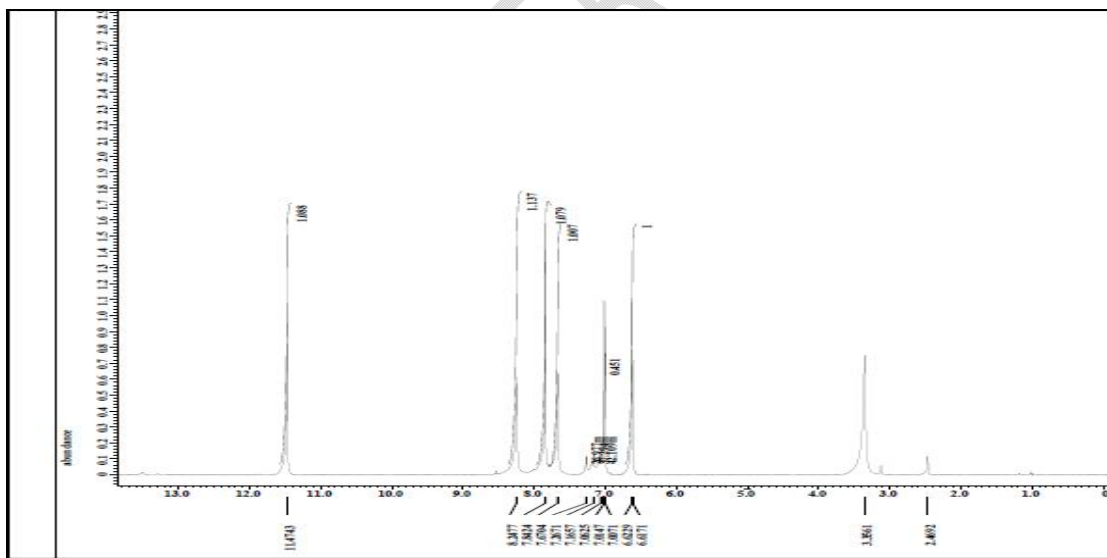
Fig(3) The 1 H NMR spectrum of (5CIPTSC)
