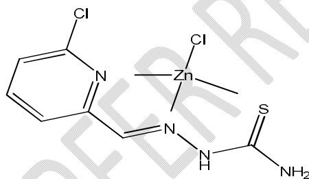
Fig (12): The probable structure of complex [Zn (HL1)2]
