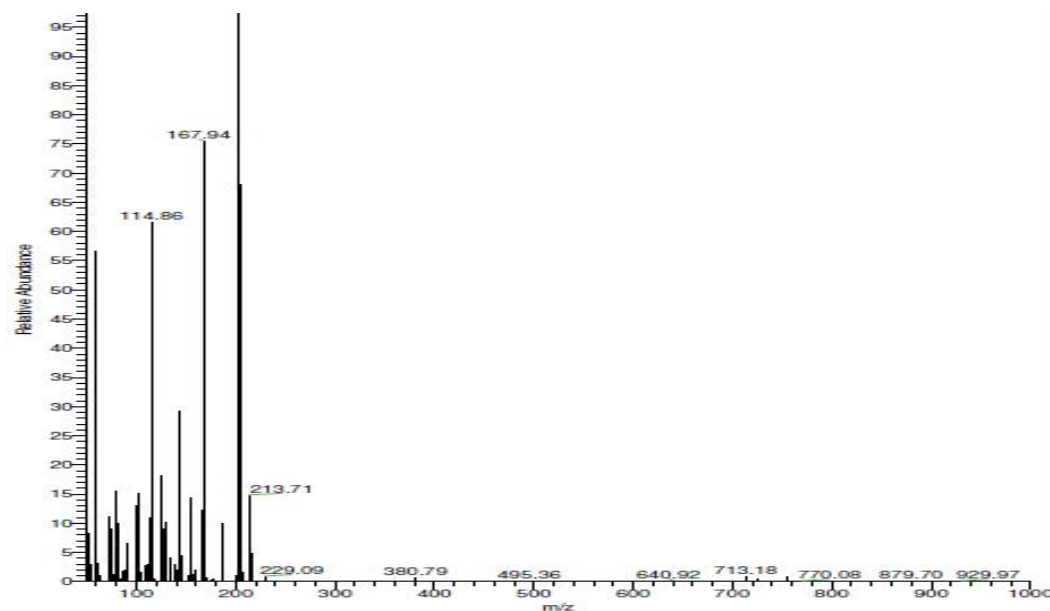
Fig(5 ) Mass spectrum of [Ni(HL1) 2 ]
