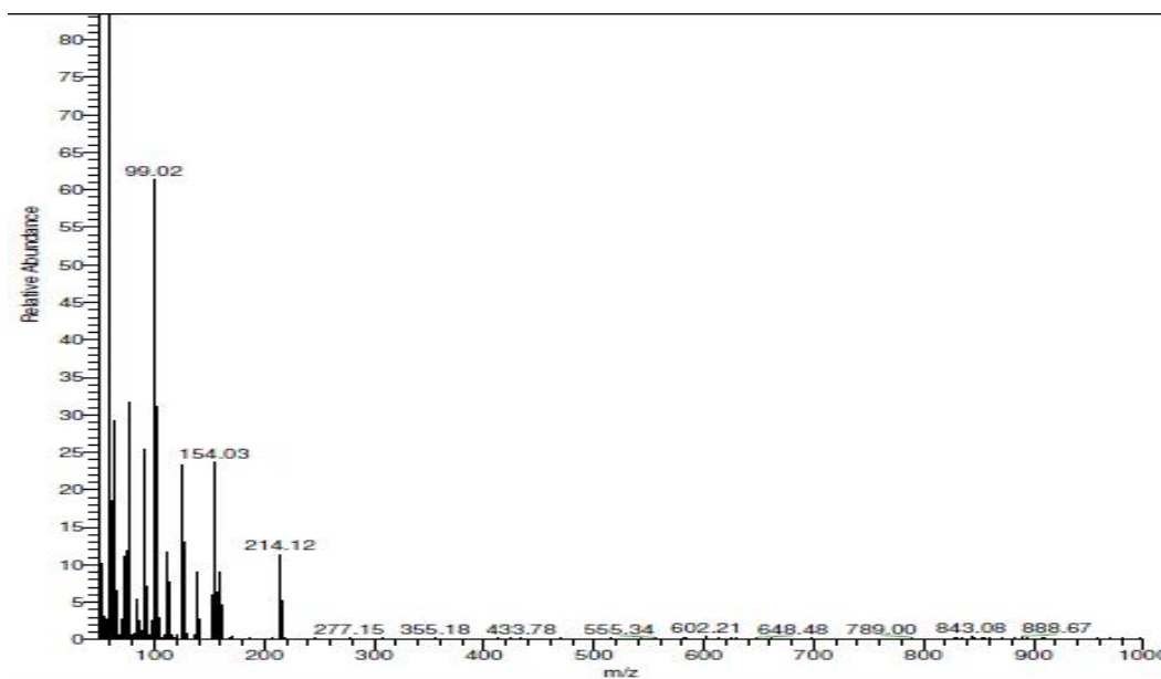
Fig(7) Mass spectrum of [Zn(HL1) 2 ]
