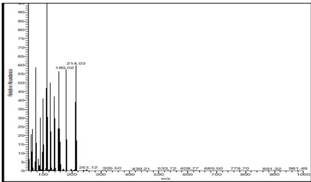
Fig(9) Mass spectrum of [Cu(HL1) 2 ]
