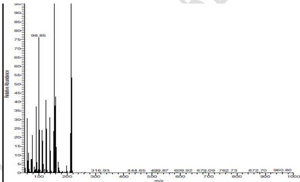
Fig(8) Mass spectrum of [Cu(HL1)]
