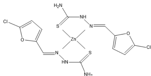
Fig(9) Structure of [Zn(C_6H_6ClN_3SO)_2]
