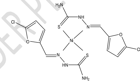
Fig(8) Structure of [\text{Ni}(\text{C}_6\text{H}_6\text{ClN}_3\text{SO})_2]
