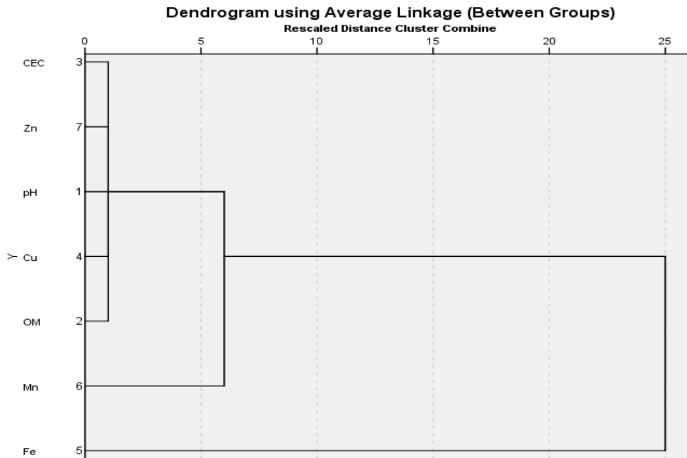
Figure 1: Hierarchical clusters soil properties determined in the studied agricultural soils.
