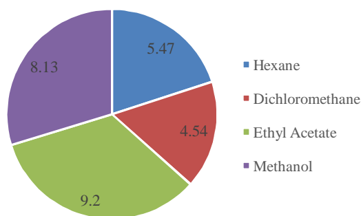
Figure 1. Fractions distribution of Vitex pubescens Vahl
