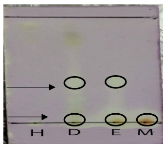
Figure 2. TLC-DPPH with the eluent of DCM-EtOAc (5:5) for V. pubescens fractions
