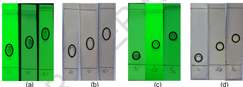
Figure 3. TLC bioautography two pure compound DCM: EtOAc with eluent (6:4, 4:6, 3:7) (a) compound 1 UV_{254} nm, (b) with DPPH reagent, (c) compound 2 UV_{254} nm dan (d) with DPPH reagent.
