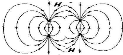
Figure 1. Conditional bidipole configuration of the " electromagnetic particle ".
