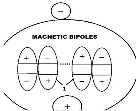
Figure 4. Conventional scheme of the hydrogen atom :
