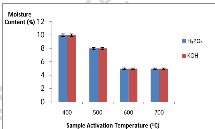
Fig. 2. Chart of Moisture Content of activated samples
