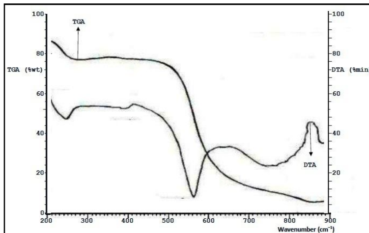
Fig. 7. TGA/DTA of the precursor sample
