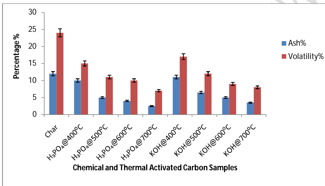
Fig. 3. Results for Percentage Ash Content and Volatility of Samples
