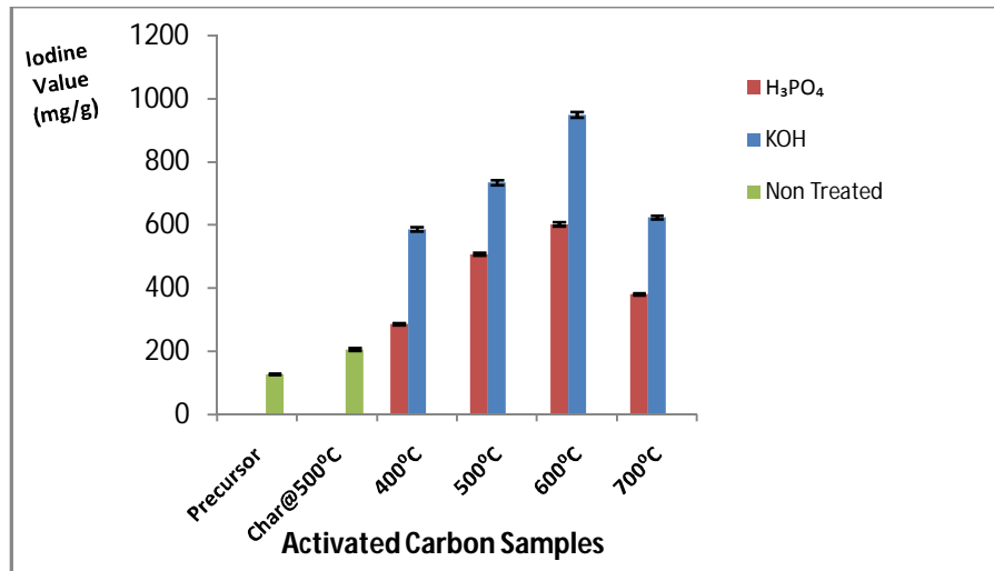
Fig. 4. Iodine Absorption Value (IV) of Samples
