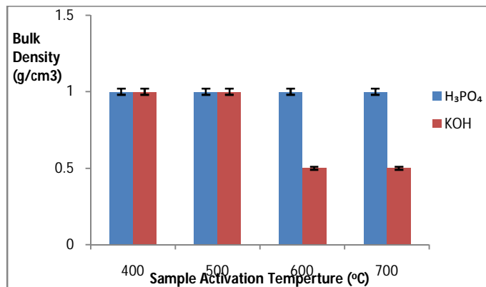
Fig. 1. Chart of Bulk Density of activated samples
