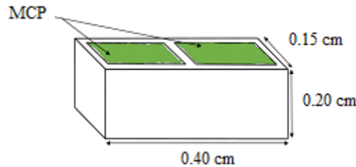
Figure 2. Cinder block hollow brick containing MCP
