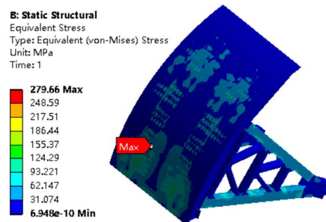
Figure 7 Overall structural stress cloud
