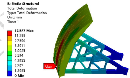
Figure 19 Overall structural displacement cloud
