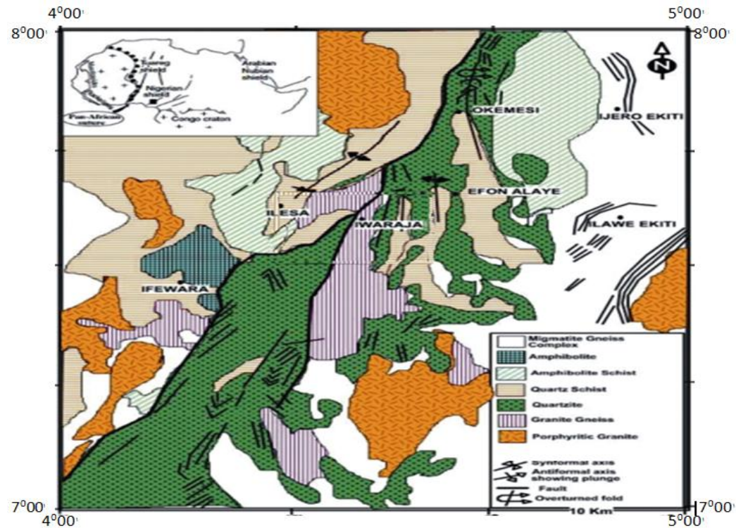
Figure 2: Geological map of the study area over Ilesha and its environment
