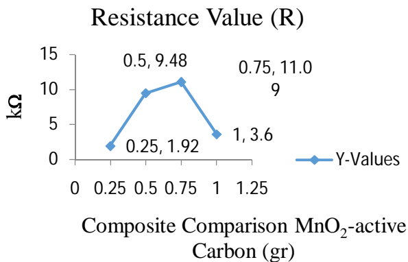
Figure 5. Resistance Value (R)
