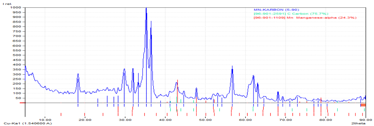
Figure 3. MnO 2 -Carbon Composite XRD Results
