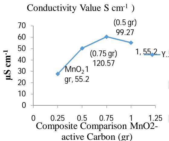
Figure 7. Conductivity Value
