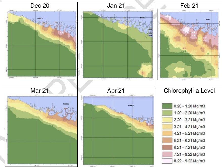
Figure 2. Chlorophyll-a Map Aru Sea December 2020 - April 2021
