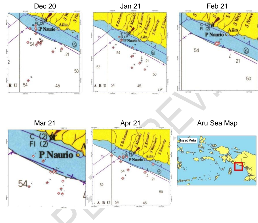
Figure 1. Fishing Areas December 2020 to April 2021
