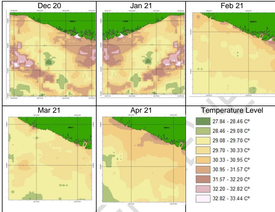
Figure 3. SST Distribution Map Aru Sea December 2020 - April 2021
