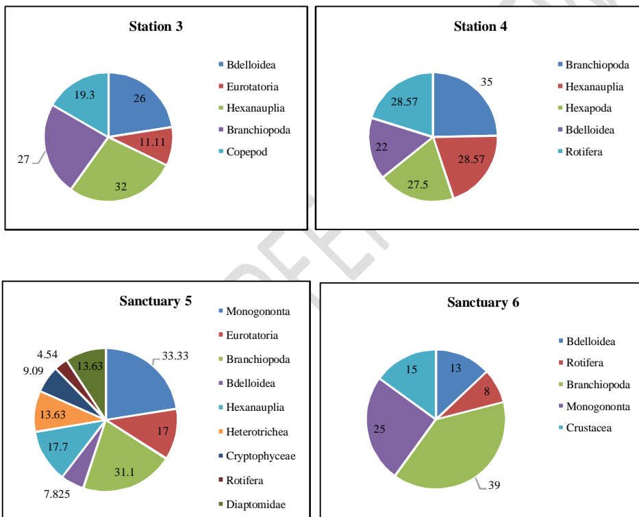
Figure 8. Zooplankton composition in seven sampling stations
