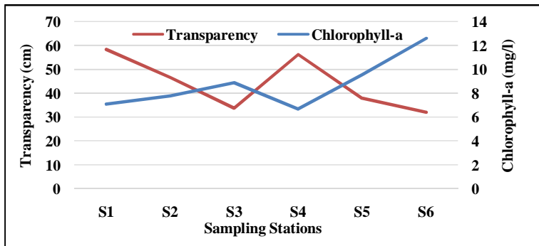
Fig.3. Variations of transparency and chlorophyll at sampling stations.
