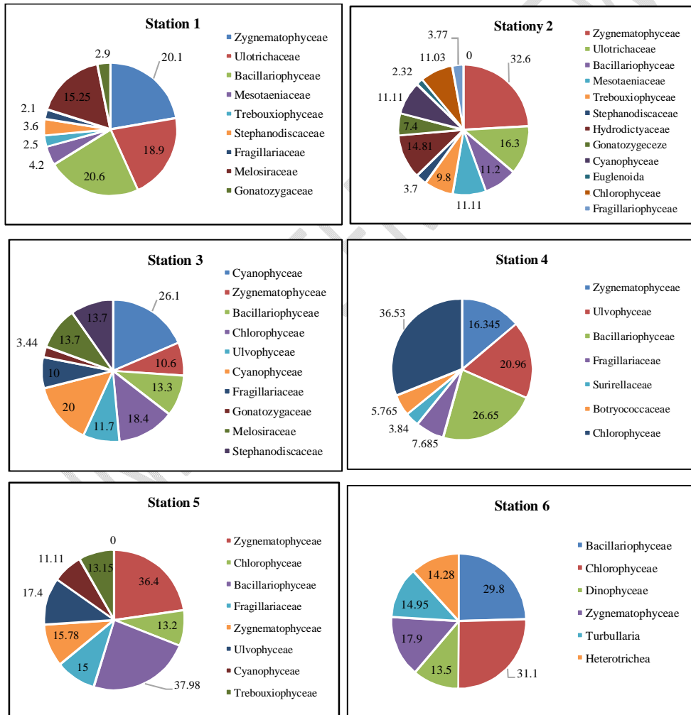
Figure 7. Phytoplankton composition in six sampling stations
