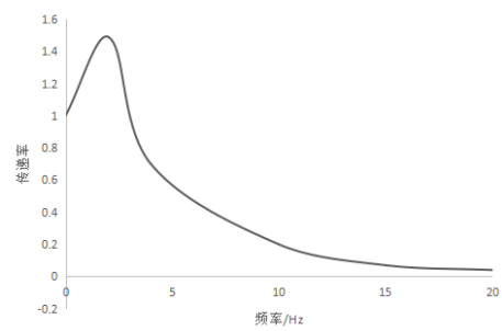
Figure 24: Simulation transfer characteristic curve of 70kg payload
