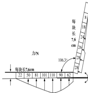
Figure 2: Reasonable distribution of forces on each part of the seat [27]
