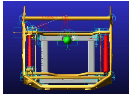
Figure 17: Shock absorber model
