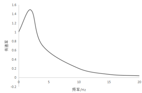
Figure 24: Simulation transfer characteristic curve of 70kg payload
