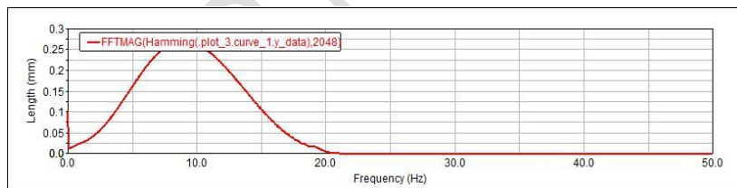
Figure 21: The Fourier transform curve of the cargo
