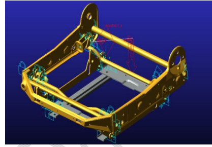
Figure 15: Constraint diagram of the virtual prototype
