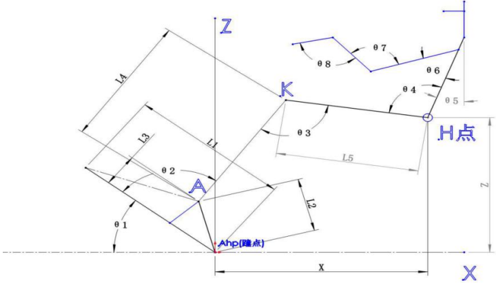
Figure 7: Human body H-point calculation model
