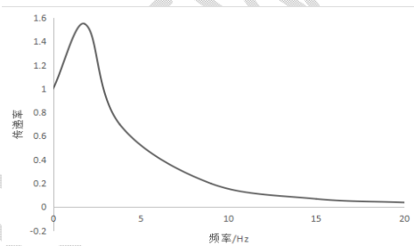
Figure 25: Simulation transfer characteristic curve of 80kg payload
