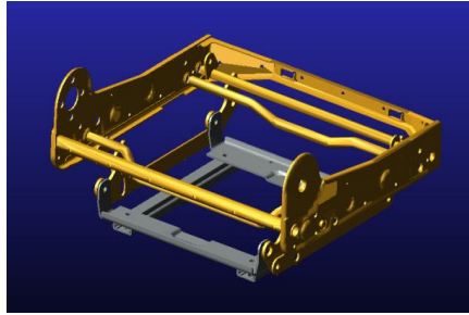
Figure 14: Simplified model of the forklift seat frame
