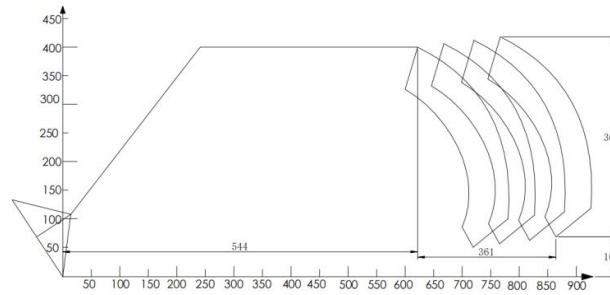
Figure 10: H-point comfortable sitting area map (different human body percentiles)
