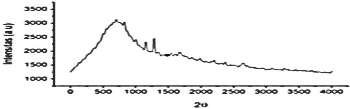
Figure 1. Activated Carbon Crystallinity Curve Using X-Ray Diffraction) Temperature 700□
