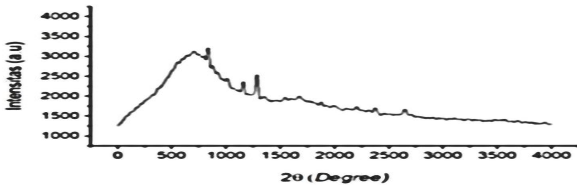
Figure 2. Activated Carbon Crystalline Curve Using X-Ray Diffraction Temperature 800□
