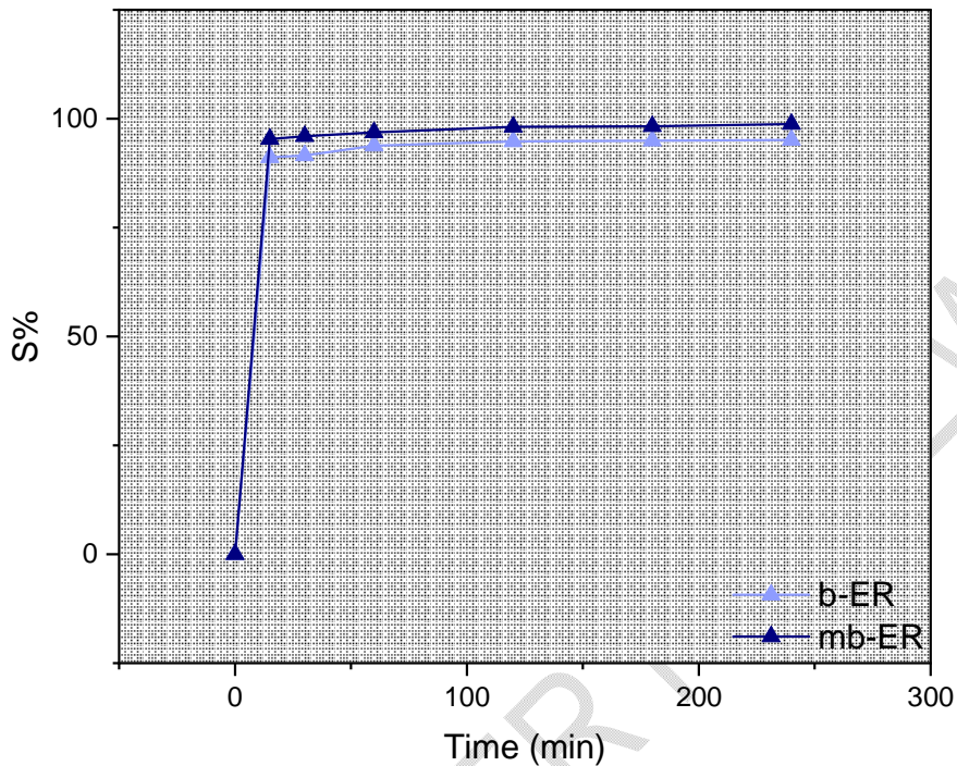
Fig. 6. Variation of sorption with contact time
