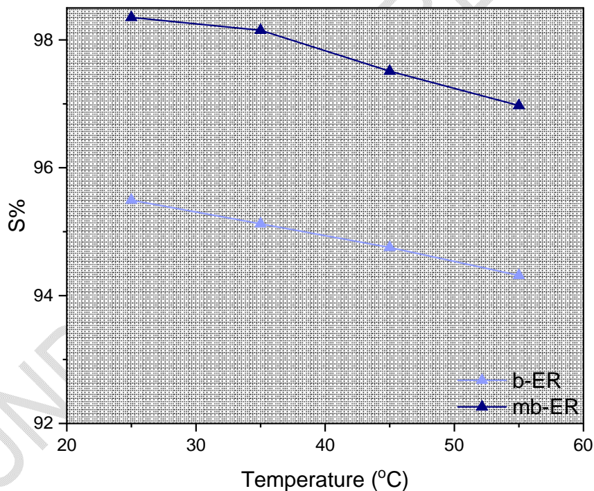
Fig. 5. Variation of sorption with temperature
