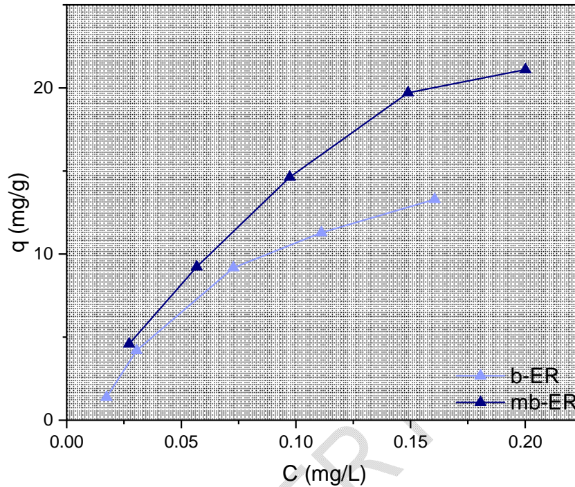
Fig. 3. Variation of adsorption capacity with equilibrium concentration
