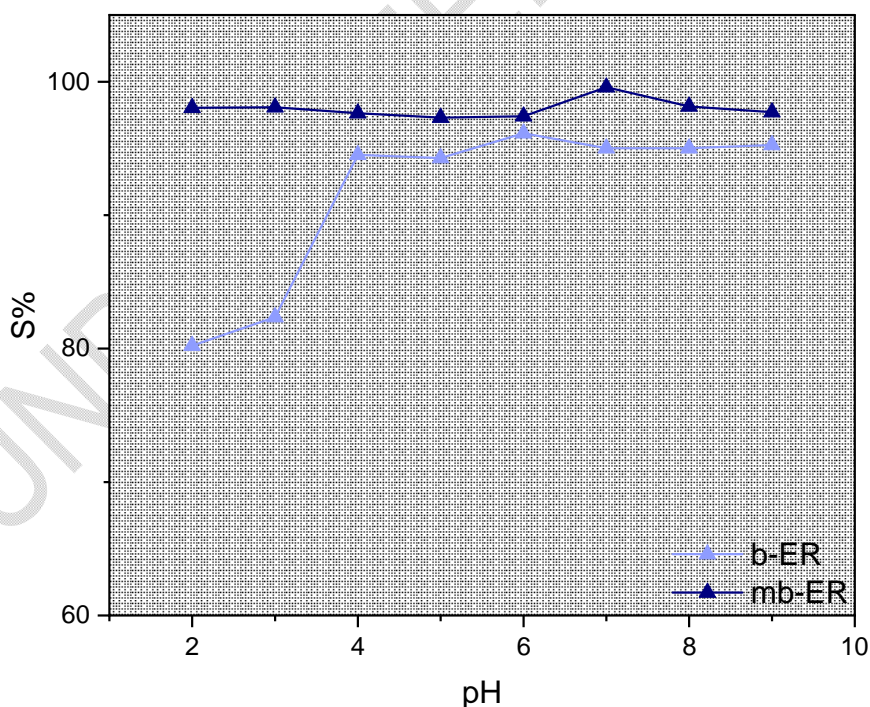
Fig. 4. Variation of sorption with pH
