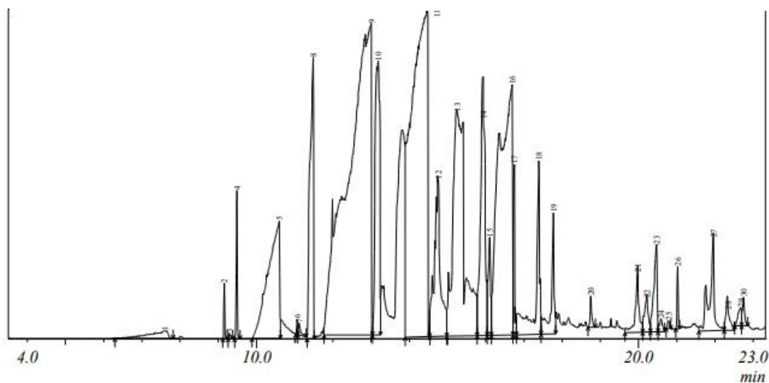
Figure 1. Chromatogram of the methanolic extract of I. gabonensis
