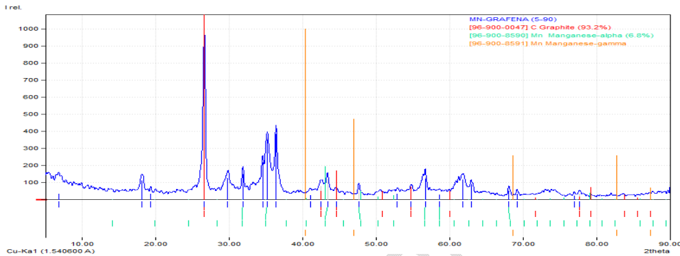
Figure 3. XRD Results of the MnO 2 -Graphene Composite
