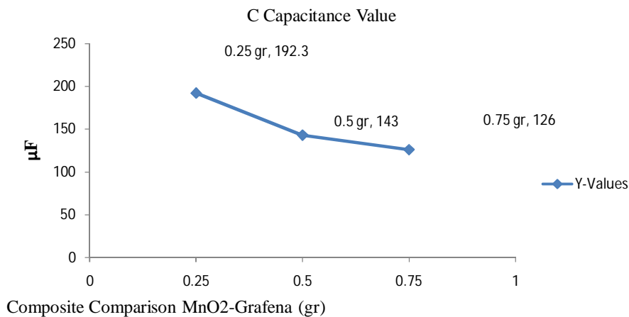
Figure 4. MnO 2 -Graphene Composite Capacitance test graph
