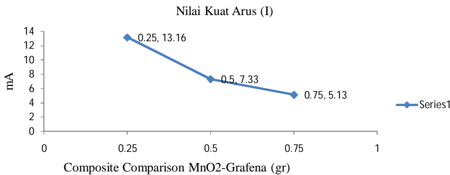
Figure 6. Graph of MnO 2 -Graphene Composite Flow Test
