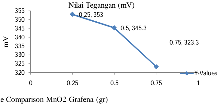
Figure 5. Graph of MnO 2 -Graphene Composite Stress test
