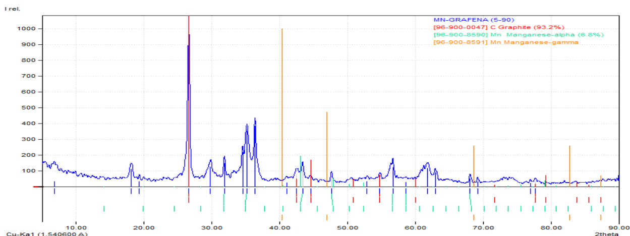
Figure 3. XRD Results of the MnO 2 -Graphene Composite
