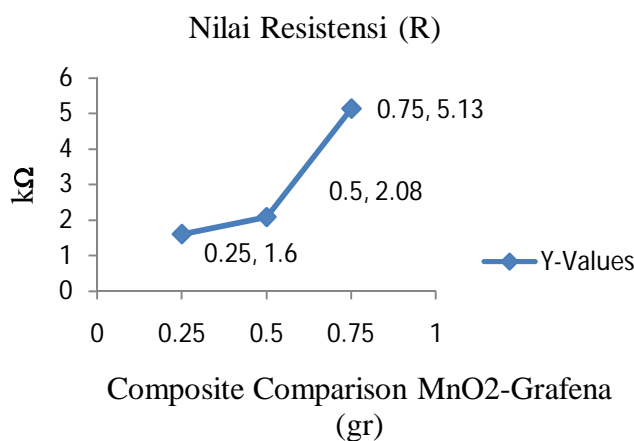
Figure 7. MnO 2 -Graphene Composite Capacitance test graph
