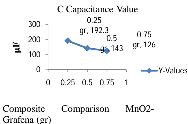
Figure 4 MnO 2 -Graphene Composite Capacitance test graph
