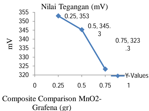
Figure 5. Graph of MnO 2 -Graphene Composite Stress test
