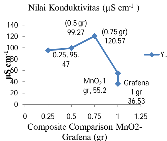
Figure 8. MnO 2 -Graphene Composite Capacitance test graph
