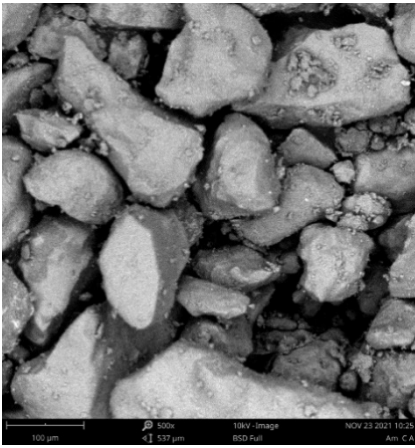
Fig. 3. SEM analysis of Amansea clay before activation (100 µm)
