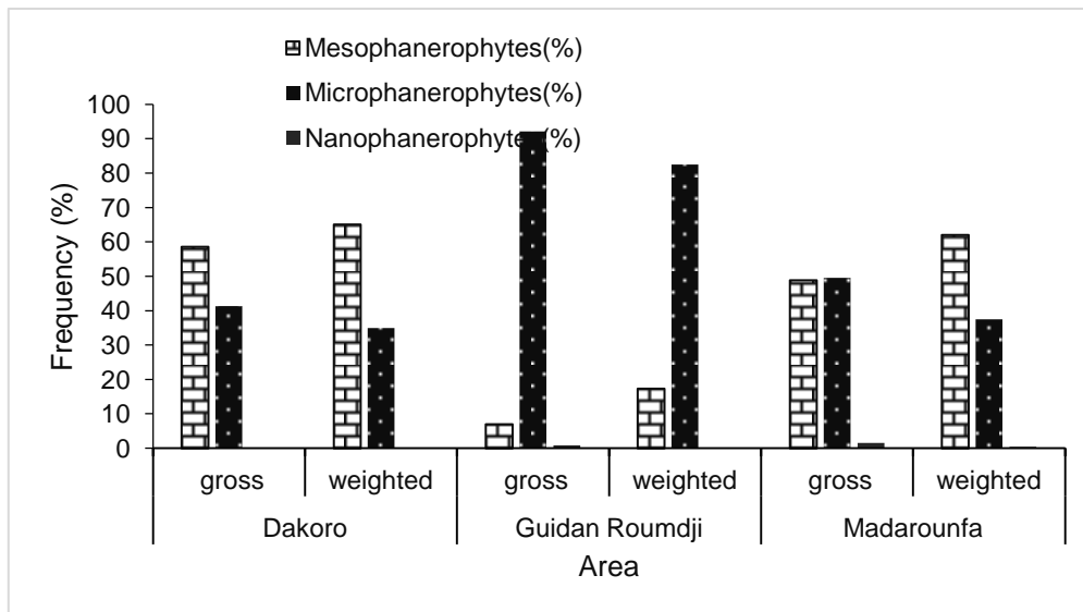
Figure 2: Frequency of raw and weighted spectra by area
