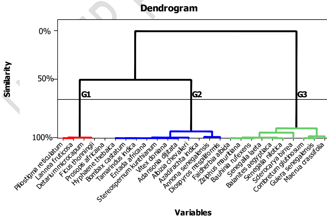
Figure 3: Correspondence factor analysis of woody species, frequency by zone Dendrogram readings
