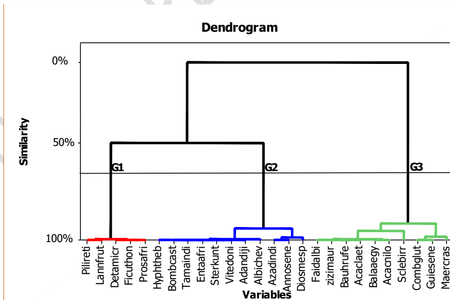
Figure 4: Hierarchical bottom-up classification of plant groupings across the study area.
