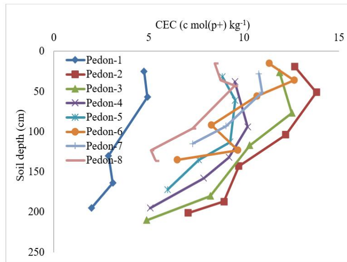
Fig. 3 Vertical distribution of CEC in different pedons
