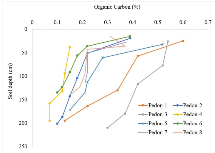
Fig. 1 Vertical distribution of organic carbon in different pedon
