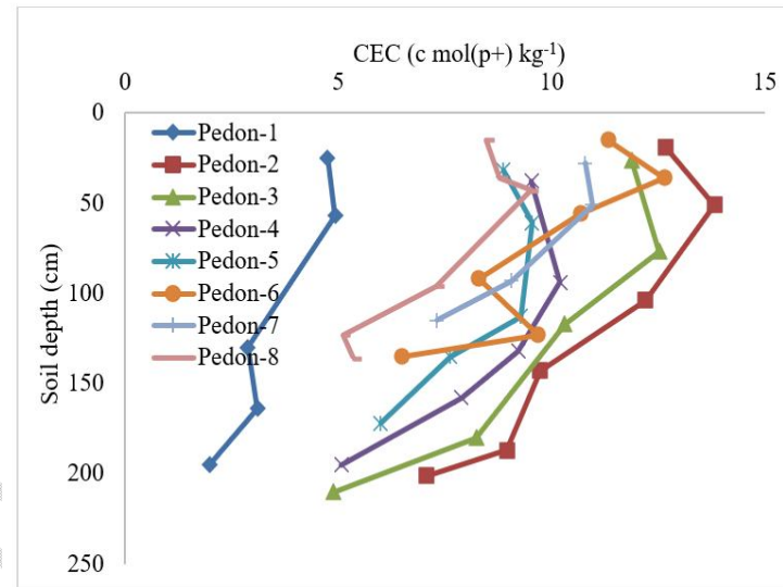
Fig. 2 Vertical distribution of CEC in different pedons
