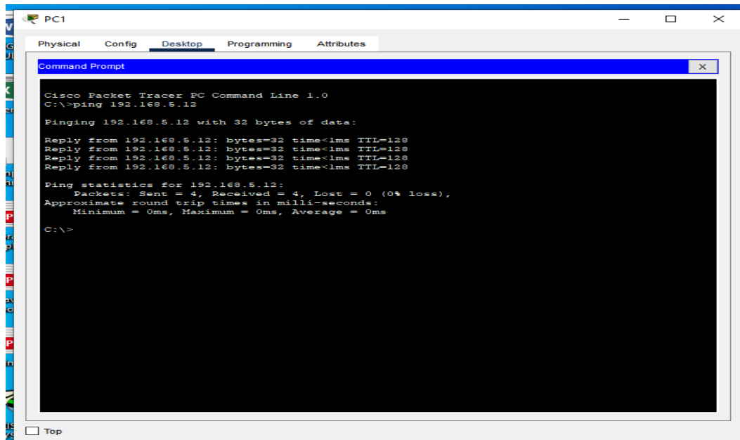
Figure 6: Successful Status of two Systems Communicating with each other on same VLAN but not on same place.
