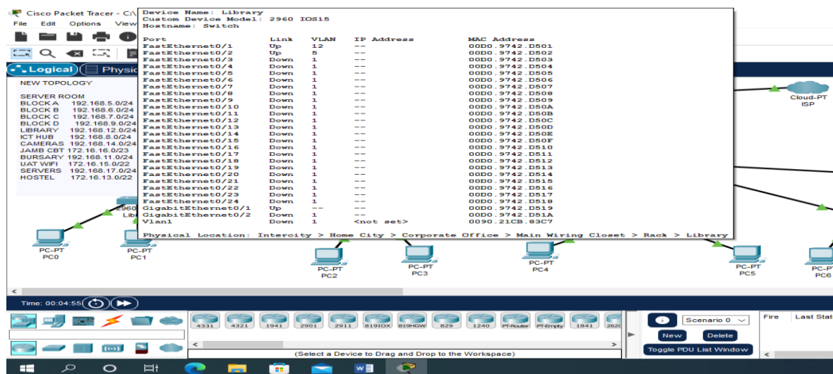
Figure 5: Shows Two Separate VLANS being configured on one Switch
