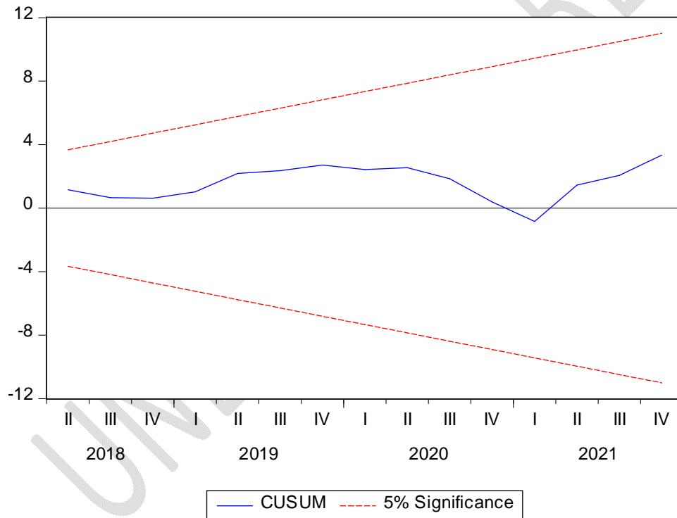
Figure1: CUSUM Test of Stability
