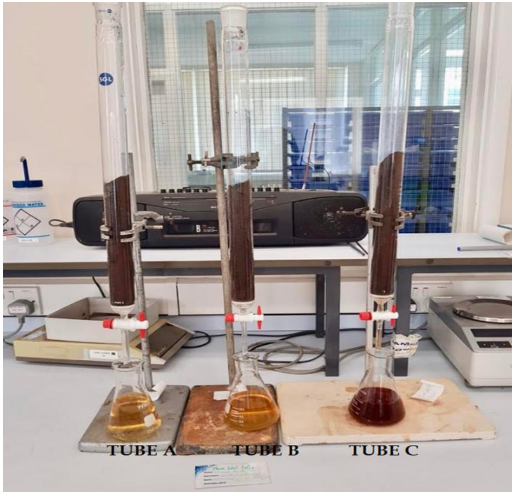
Figure 1: Experimental set-up employed in the study
