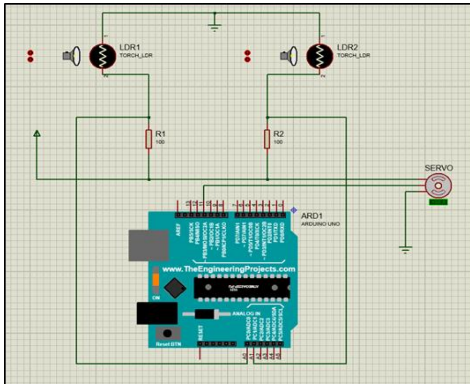
Fig.3. Experimental setup of the proposed system
