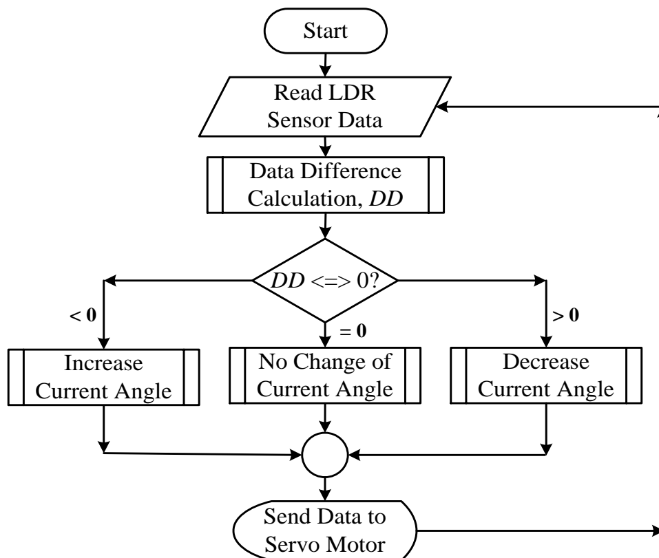
Fig.2. Flow chart of the program for the proposed system
