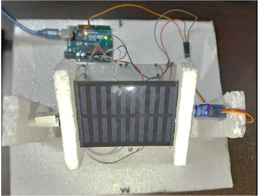
Fig.8. The servo motor rotates in the anti-clockwise direction
