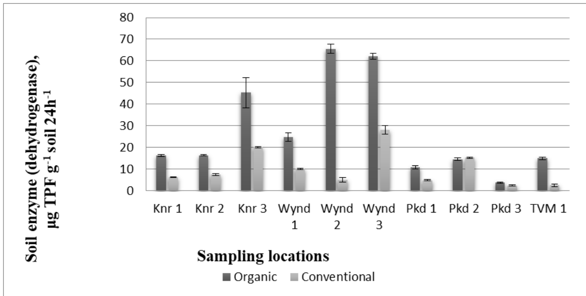
Fig 1. Effect of organic farming on soil enzyme (dehydrogenase), \mu\text{g TPF g}^{-1}\text{ soil } 24\text{h}^{-1}
