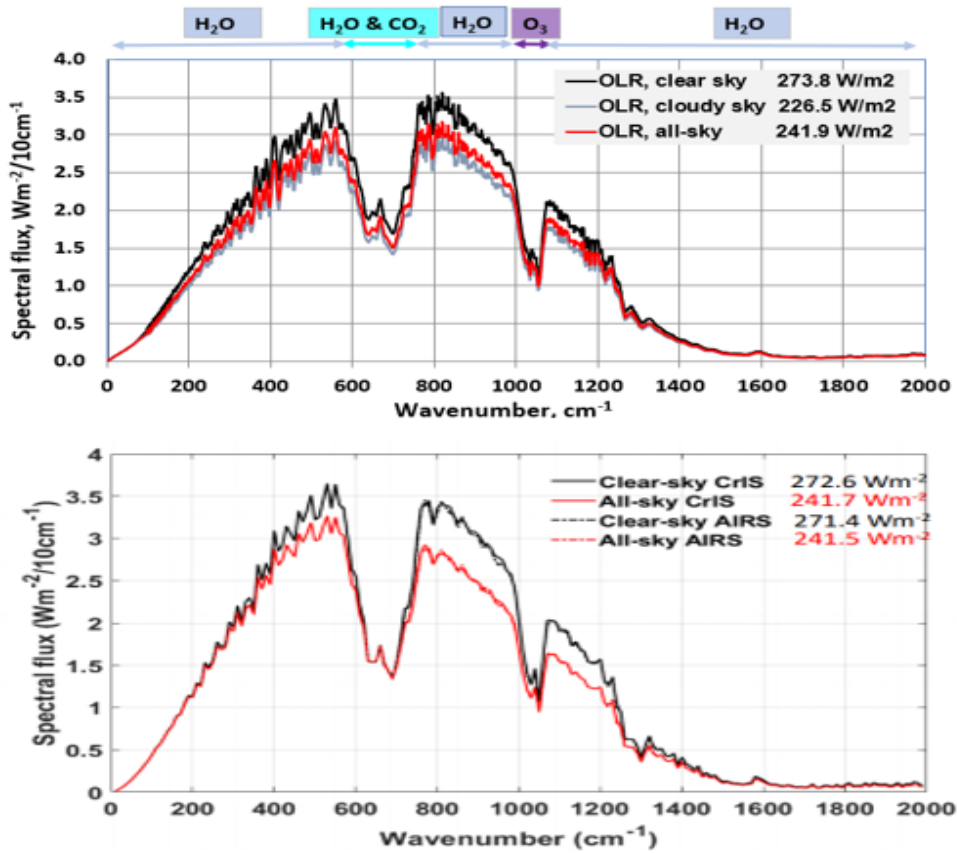
Figure 9. OLR spectral fluxes at the TOA according to the LBL calculations of this study (A), and according to observed NOAA spectral fluxes (B)[41]. Permission to reproduce Fig. 8B has been requested from Prof. Xianglei Huang.
