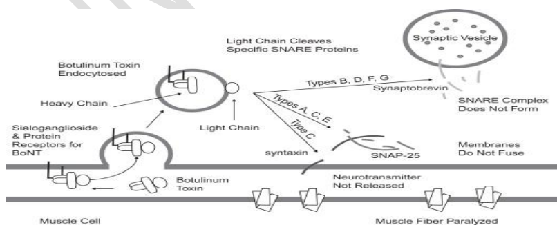
Figure1 (a, b):Mechanismofactionofbotulinumtoxin,
