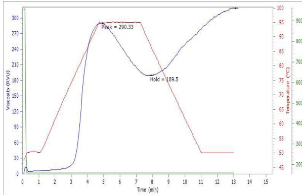
Figure 5: Viscosity flow curve of sample A1 Figure 6: Viscosity flow curve of sample A2
