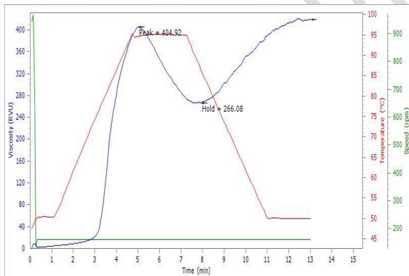
Figure 15: Viscosity flow curve of sample B9
