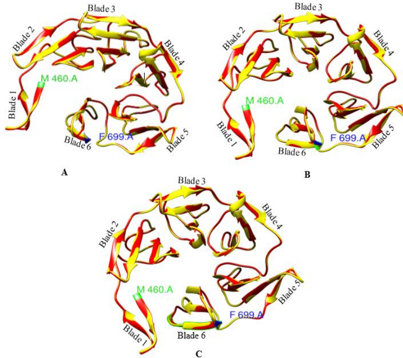
Figure 5 The 3D Structural Alignments of PfKelch13 Proteins with the Wild Type (4ZGC.1.A) Structural alignments of samples 26, 28, and 29 (represented as A, B, and C) with the wild type (4ZGC.1.A). Predicted structures are in yellow, while the reference (wild type) structures are in red. Note: M denotes Methionine; F denotes Phenylalanine.
