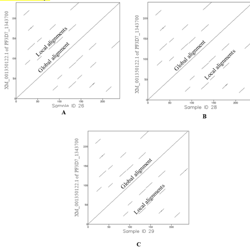
Figure 2 Dot-matcher Plot Illustrating Diversity Analysis of PfKelch13 Amino Acid Sequences
