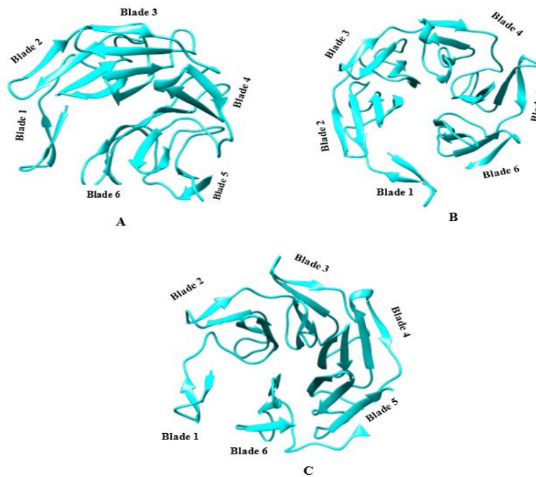
Figure 4 Predicted 3D Protein Structures of PfKelch13 genes of Samples 26, 28, and 29 Predicted 3-dimensional protein structures of samples 26, 28, and 29, represented as A, B, and C respectively. Predictions were based on the reference PDB protein structure of 4ZGC.1.A.
