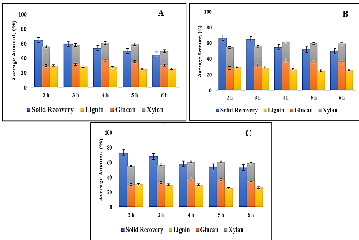
Figure 3: Composition of CS pretreated with neat solvent (A), 2.5 % diluted-solvent (B) and 5 % diluted-solvent (C) at 150 ° C.
