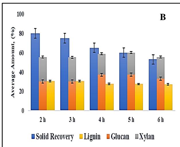
Figure 2: Composition of CS pretreated with neat solvent (A), 2.5 % diluted-solvent (B) and 5 % diluted-solvent (C) at 140 0 C.
