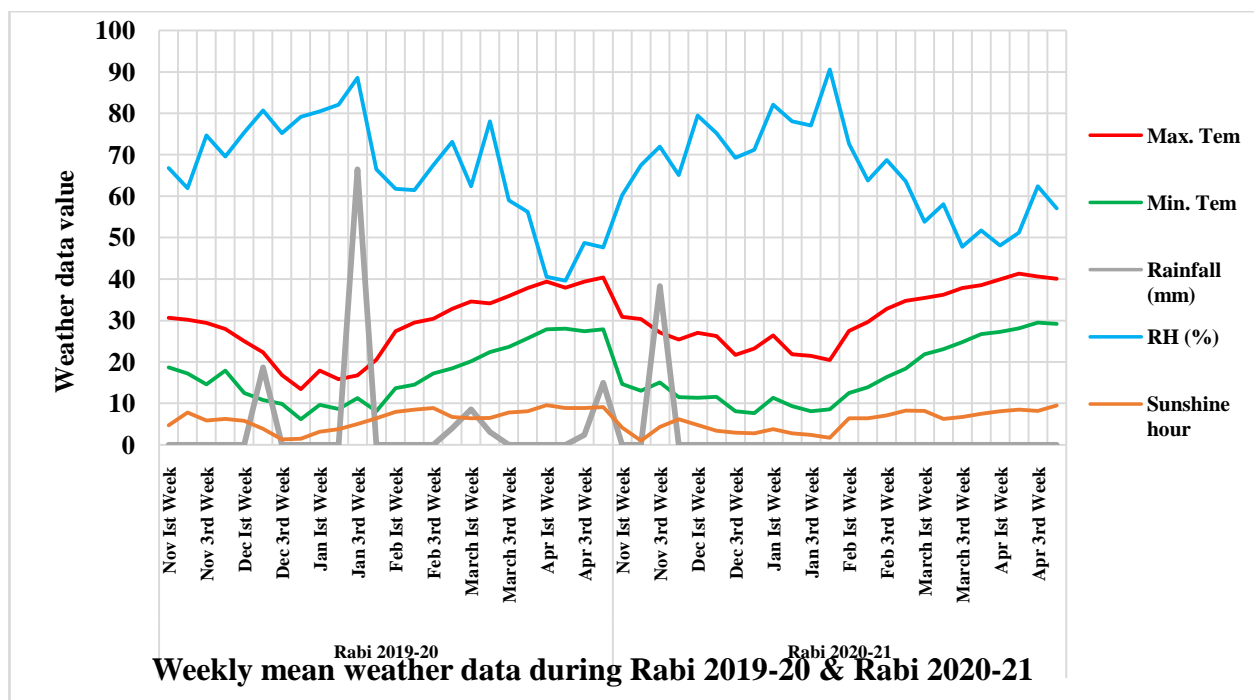
Fig. 1 Weekly min and max temp, rainfall, relative humidity (%), and sunshine hours
