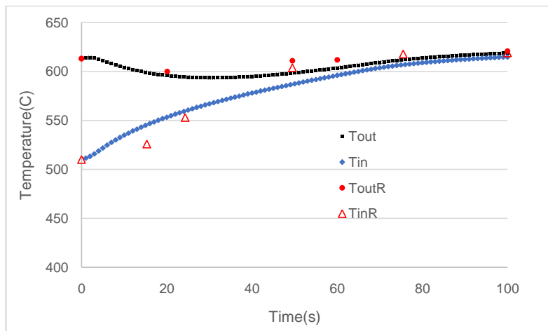
(a) Fuel salt temperatures
