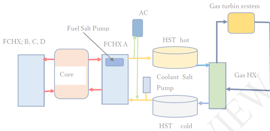
Figure 7. Schematic of a referenced conceptual molten chloride fast reactor [5]; Reproduced by the authors
