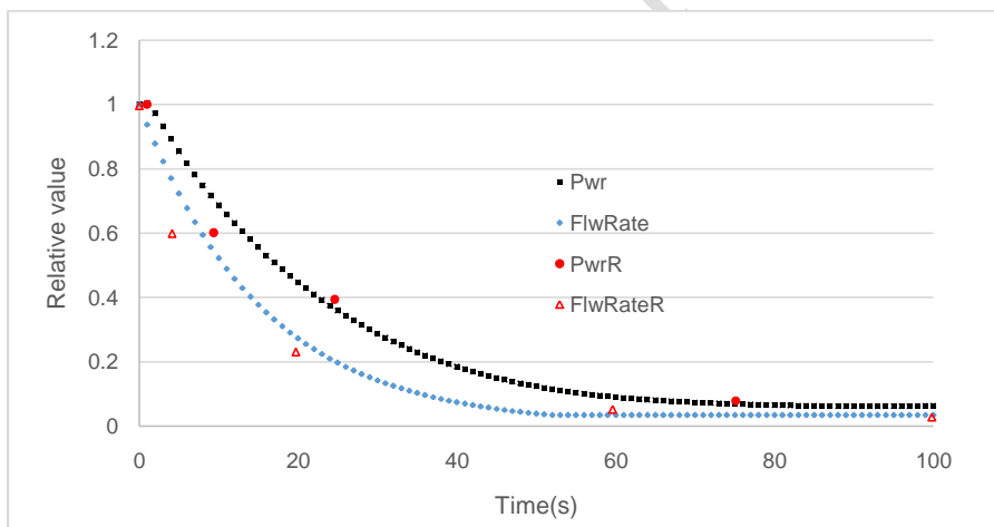
(b) Relative power and fuel flow-rate
