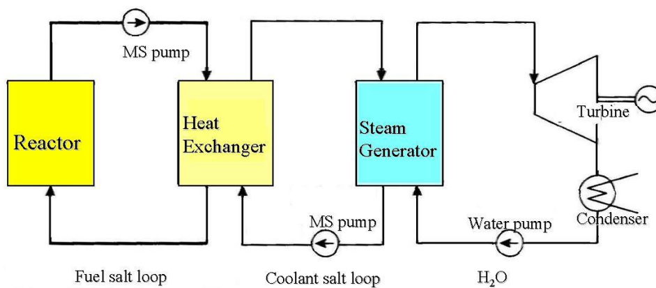
Figure 1 DYMO model for MSR power plants [18, 19, 20]
