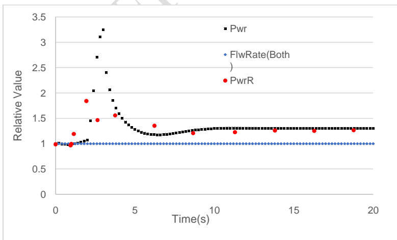
(b) Relative power and flow-rate
