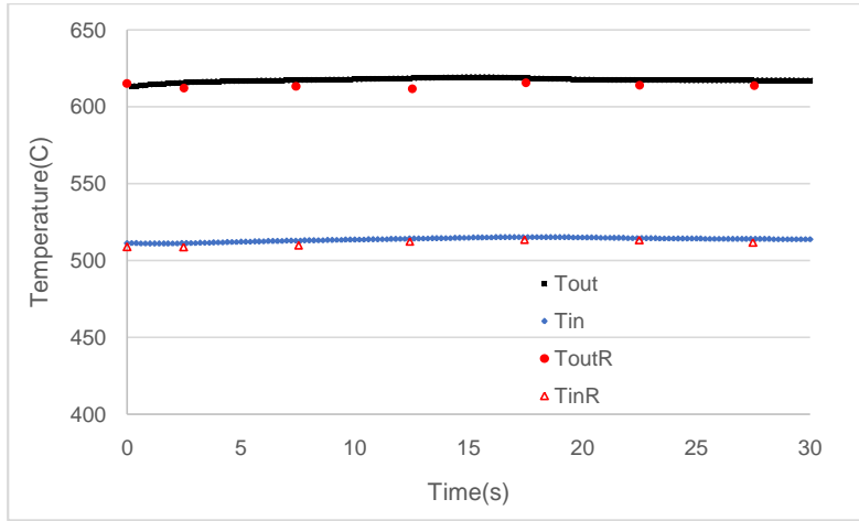
(a) Fuel salt temperatures
