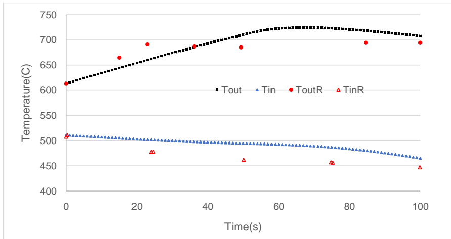
(a) Fuel salt temperature
