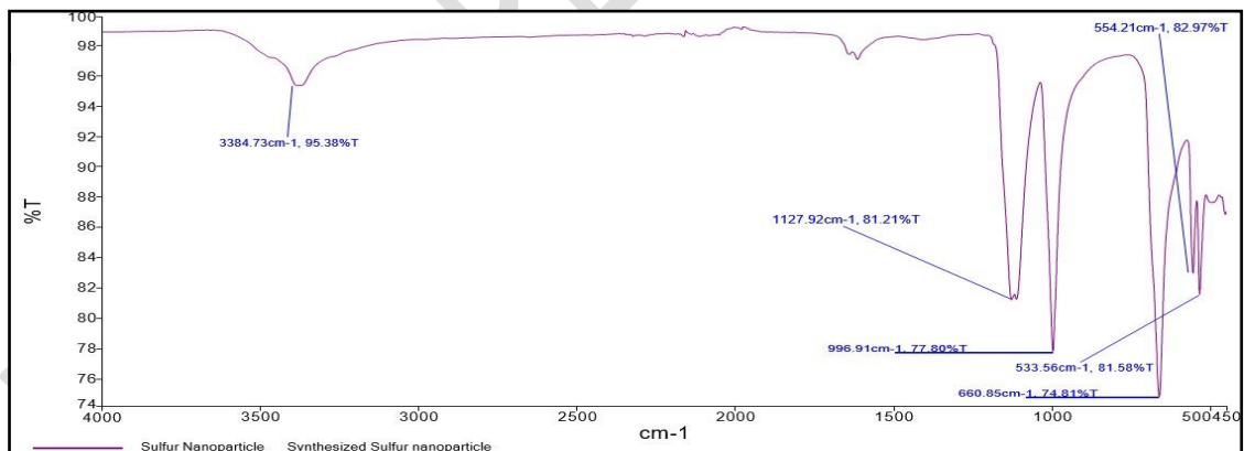
Fig. 4: FTIR spectrum of sulphur nanoparticles
