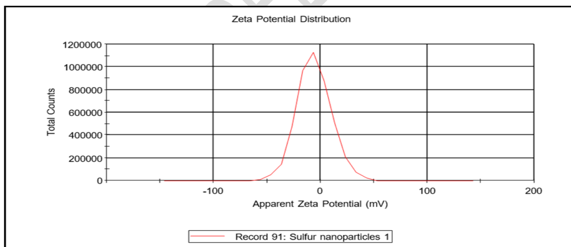
Fig.2: Zeta potential of synthesized SNPs
