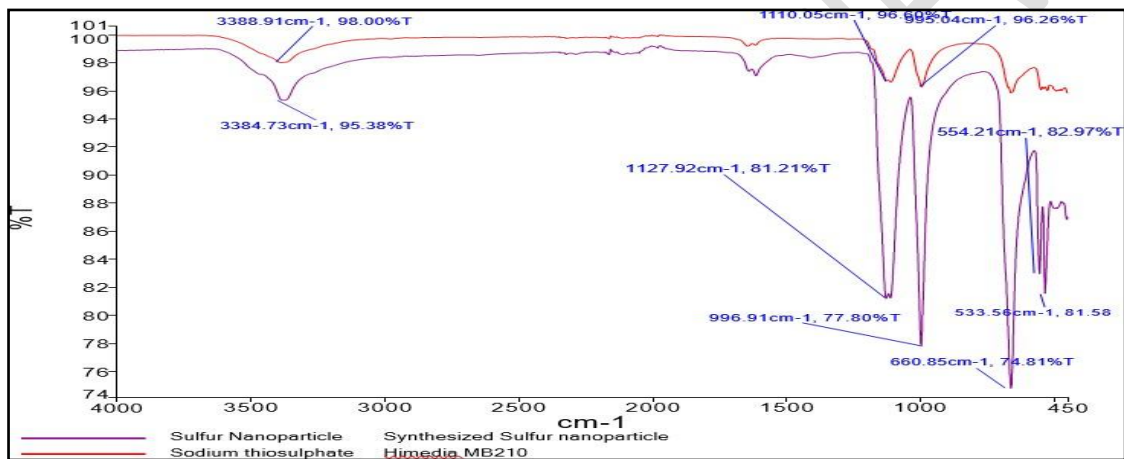
Fig. 6 Compared FTIR spectrum of sodium thiosulphate and sulphur nanoparticles
