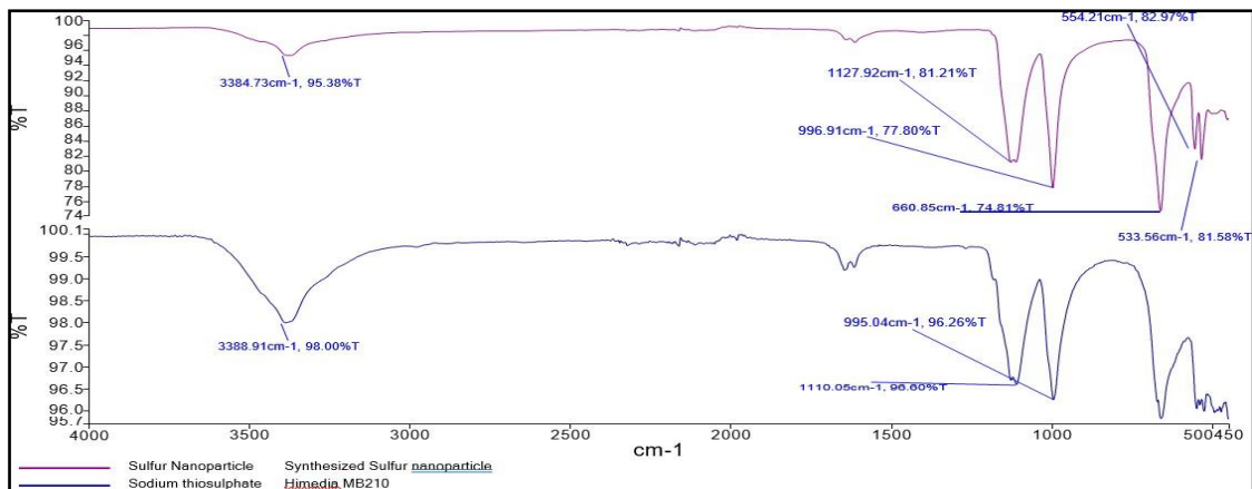
Fig. 5: Combined FTIR spectrum of sodium thiosulphate and sulphur nanoparticles
