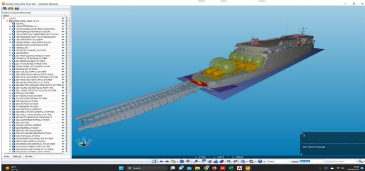
Fig – 7 Cadmatic eBrowser applications installed with MV Uhuru II 3D drawings
