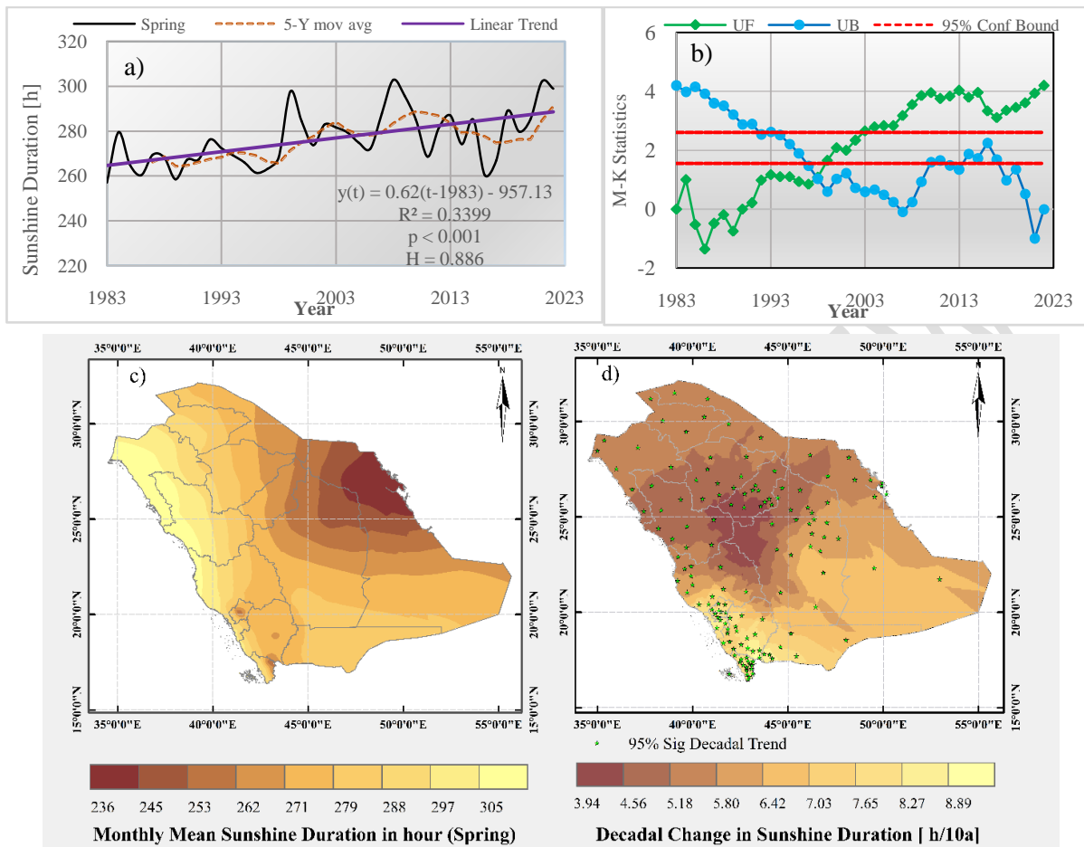
Figure 3: Variation of SD in Saudi Arabia during the Spring Season a) Sunshine duration (h) overlaid with five-year (5 - Y) moving average (red dotted) and linear trend (purple). b) M-K statistics UF (green), UB (blue) region between dotted red lines is 95% conf bond. c) Monthly mean SD in hours during spring d) Decadal trend in SD (h/10y)
