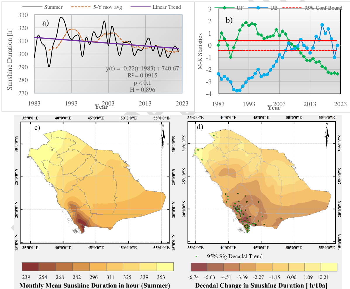
Figure 4: Variation of SD in Saudi Arabia during the Summer Season a) Sunshine duration (h) overlaid with five-year (5 - Y) moving average (red dotted) and linear trend (purple). b) M-K statistics UF (green), UB (blue) region between dotted red lines is 95% conf bond. c) Monthly mean SD in hours during summer d) Decadal trend in SD (h/10y)
