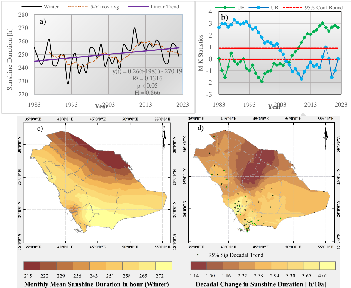
Figure 6: Variation of SD in Saudi Arabia during the Winter Season a) Sunshine duration (h) overlaid with five-year (5 - Y) moving average (red dotted) and linear trend (purple). b) M-K statistics UF (green), UB (blue) region between dotted red lines is 95% conf bond. c) Monthly mean SD in hours during winter d) Decadal trend in SD (h/10y)
