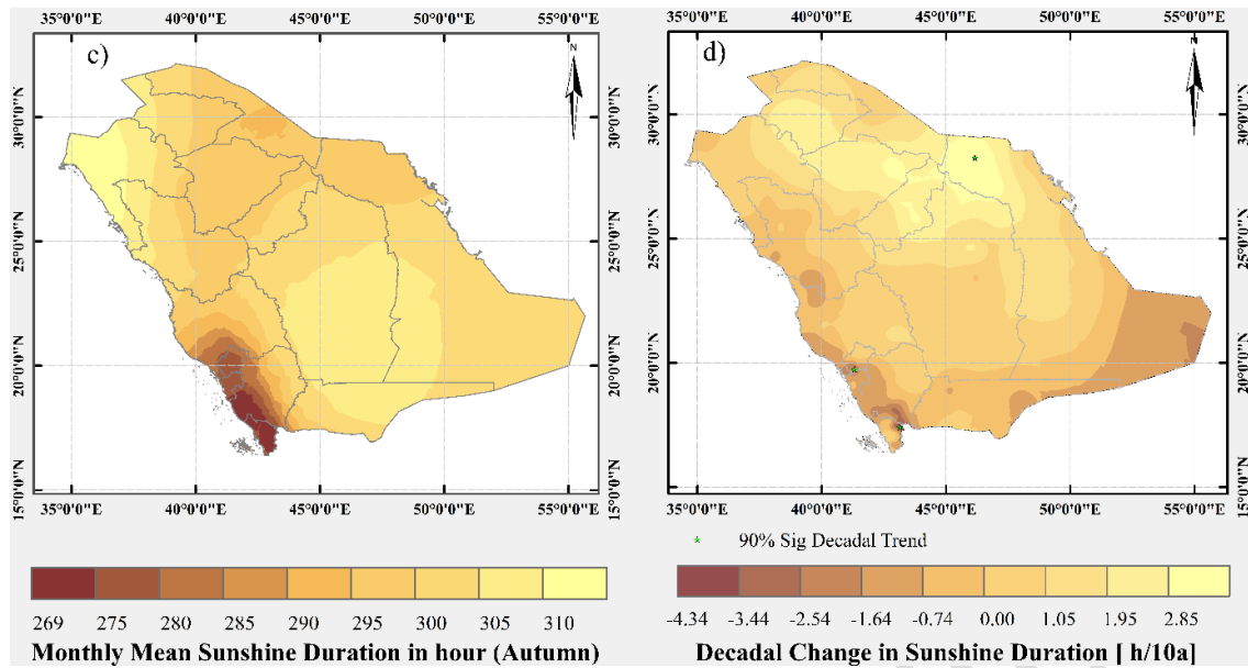
Figure 5: Variation of SD in Saudi Arabia during the Autumn Season a) Sunshine duration (h) overlaid with five-year (5 - Y) moving average (red dotted) and linear trend (purple). b) M-K statistics UF (green), UB (blue) region between dotted red lines is 95% conf bond. c) Monthly mean SD in hours during autumn d) Decadal trend in SD (h/10y)
