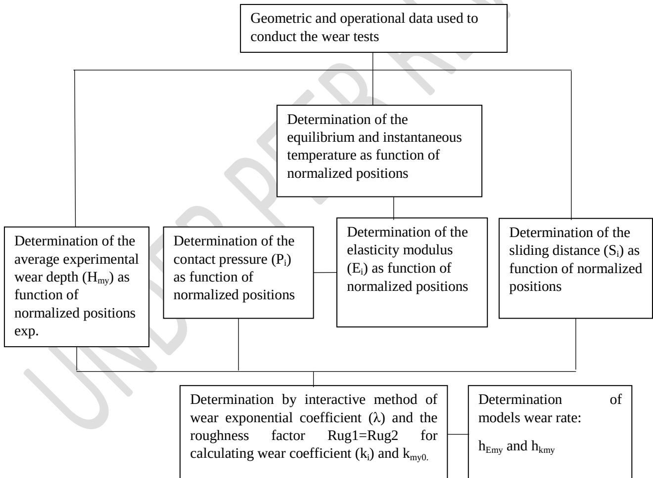
Figure 5- Flowchart for the simulation
