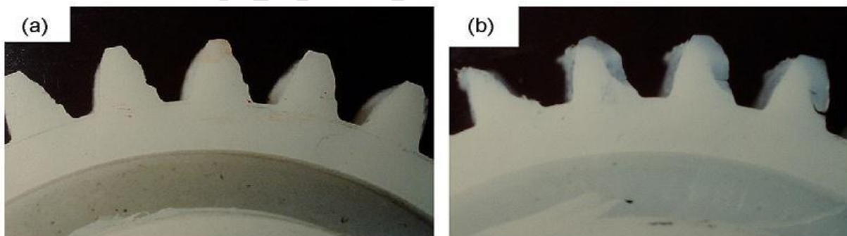
Figure 2- Acetal gear wear forms under loads of (a) 7 Nm and (b) 10 Nm [9].
