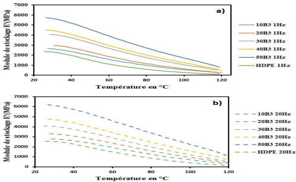
Figure 4- Storage modulus E' with different wood fiber (birch) rates for frequencies a) 1Hz and b) 20Hz as a function of temperature.
