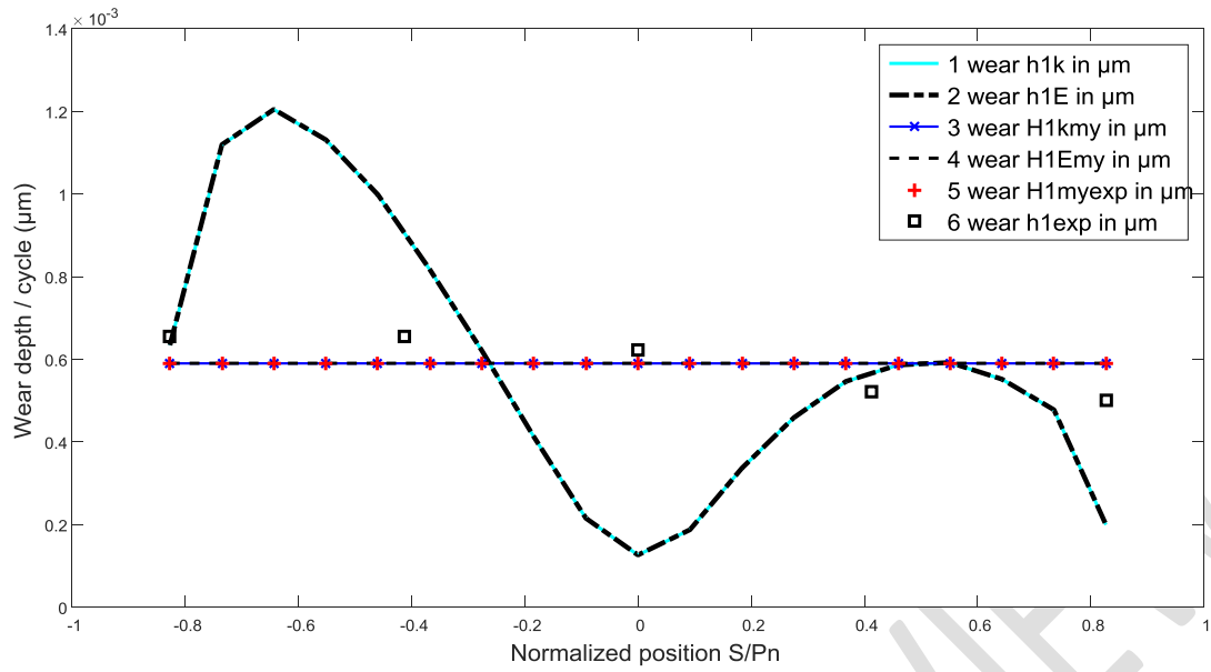
Figure 14-Evolution of the wear rate experimental and models according to the s/pn positions; driver gear wheel; torque 5Nm; speed 1000 rpm.
