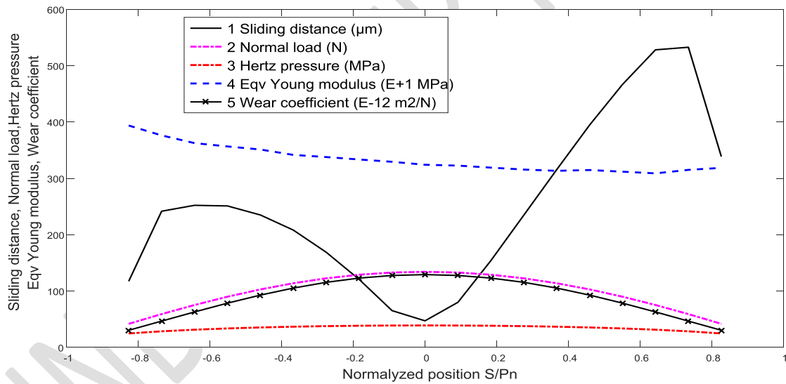
Figure 7- Evolution according to the normalized position of the sliding distance, the normal load, the Hertz pressure, the equivalent Young's modulus, and the wear coefficient of the driver gear: HDPE30B/HDPE30B ; C = 5\text{Nm} , \omega = 1000\text{rpm} ; exponential wear coefficient \lambda = 2.8865 .
