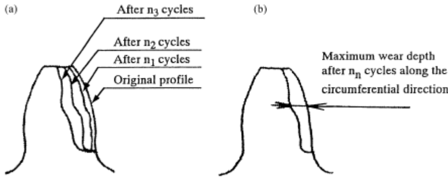
Figure 3- Schematic drawings of tooth profile change (a) and measurement of wear depth (b) [13].
