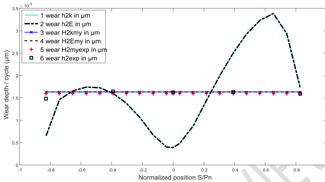
Figure 11- Evolution of the wear rate experimental and models according to the s/pn positions, driven gear wheel, torque 6Nm, speed 500 rpm.
