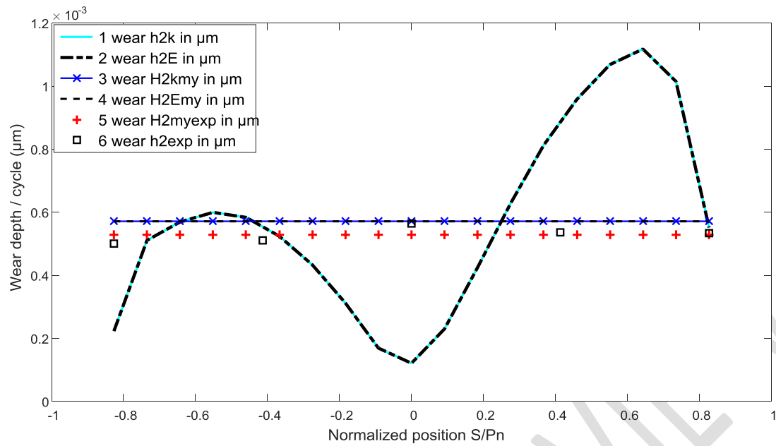
Figure 10- Evolution of the wear rate experimental and models according to the s/pn positions, driven gear wheel, torque 5Nm, speed 1500 rpm.
