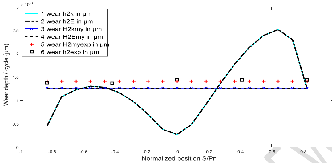
Figure 8- Evolution of the wear rate experimental and models according to the s/pn positions, driven gear wheel, torque 5Nm, speed 500 rpm.
