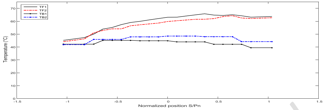
Figure 6- Evolution according to the normalized position of the equilibrium temperatures TB1, TB2 and the instantaneous temperatures TF1, TF2 for the driver and the driven gears: HDPE30B/HDPE30B ; C = 5\text{Nm} ( \text{Phmoy} = 34.33\text{ MPa} ), \omega = 1000\text{rpm} .
