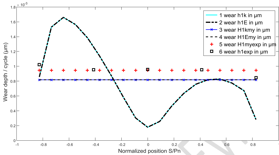
Figure 13- Evolution of the wear rate experimental and models according to the s/pn positions; driver gear wheel; torque 5Nm; speed 500 rpm.
