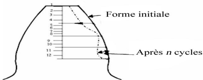
Figure 1- Change in tooth shape with wear [11].
