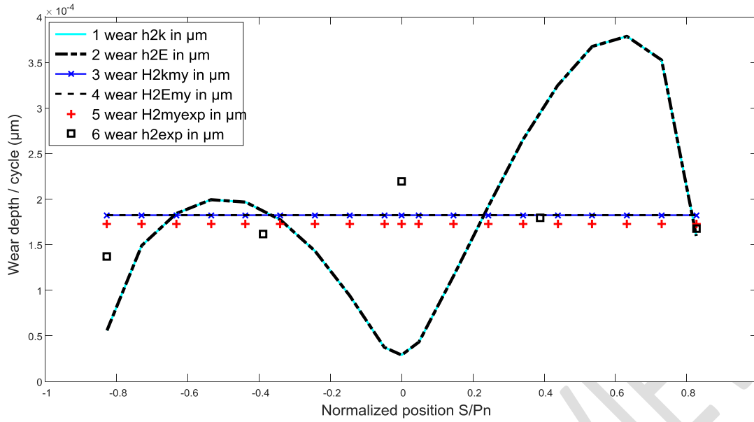
Figure 12-Evolution of the wear rate experimental and models according to the s/pn positions, driven gear wheel, torque 2Nm, speed 1000 rpm.
