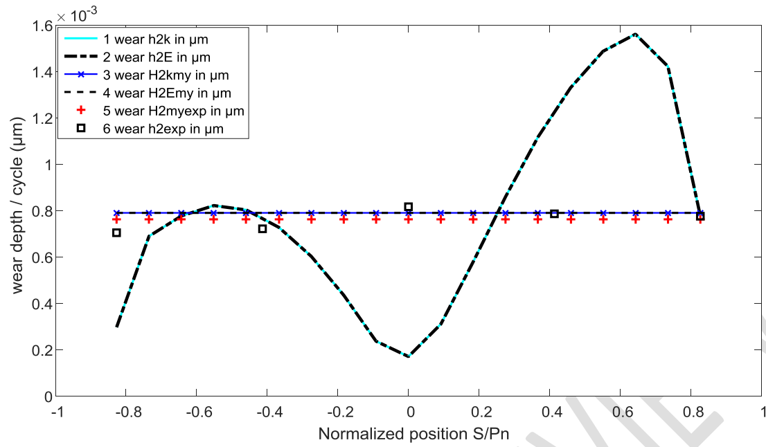
Figure 9- Evolution of the wear rate experimental and models according to the s/pn positions, driven gear wheel, torque 5Nm, speed 1000 rpm.
