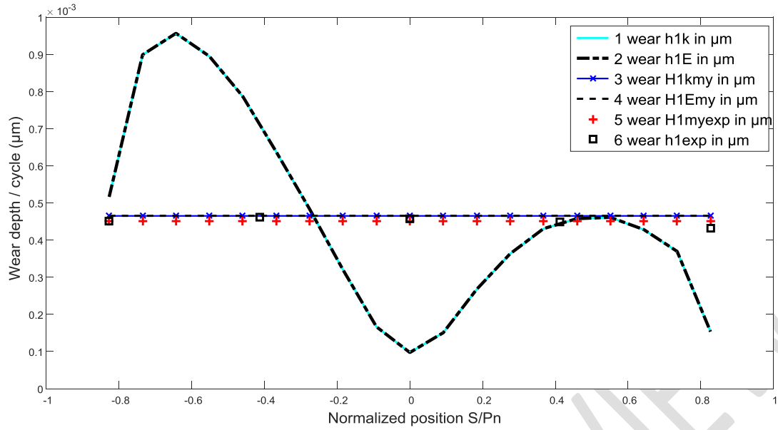
Figure 15-Evolution of the wear rate experimental and models according to the s/pn positions; driver gear wheel; torque 5Nm; speed 1500 rpm.
