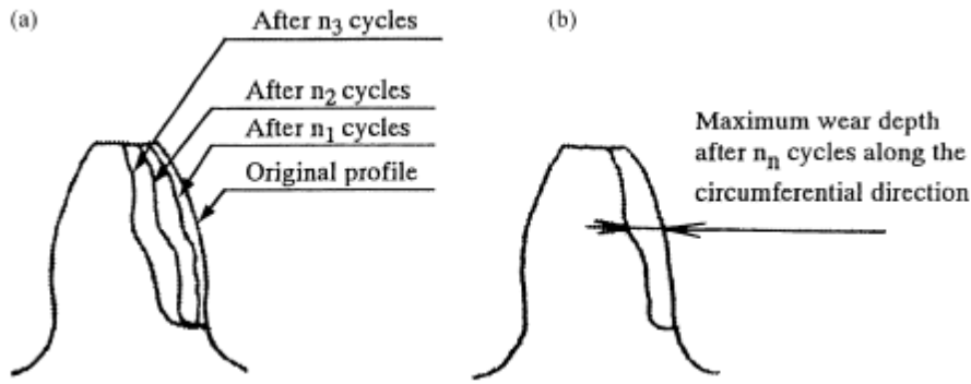
Figure 3- Schematic drawings of tooth profile change (a) and measurement of wear depth (b) [13].
