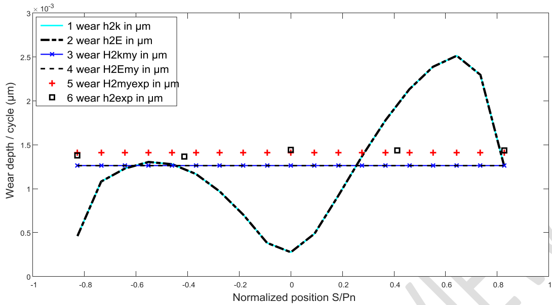
Figure 8- Evolution of the wear rate experimental and models according to the s/pn positions, driven gear wheel, torque 5Nm, speed 500 rpm.
