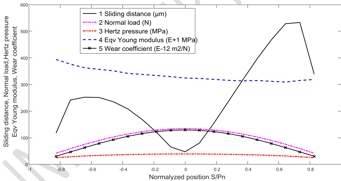
Figure 7- Evolution according to the normalized position of the sliding distance, the normal load, the Hertz pressure, the equivalent Young's modulus, and the wear coefficient of the driver gear: HDPE30B/HDPE30B ; C = 5Nm , \omega = 1000rpm ; exponential wear coefficient \lambda = 2.8865 .
