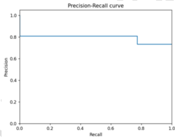
Fig 5: Precision-Recall Curve
