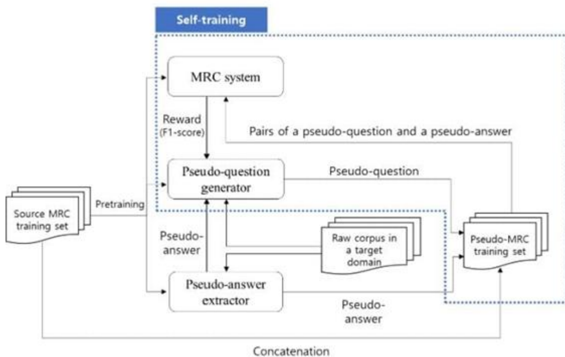
Chart 1: Framework for self-trained pseudo question generator
