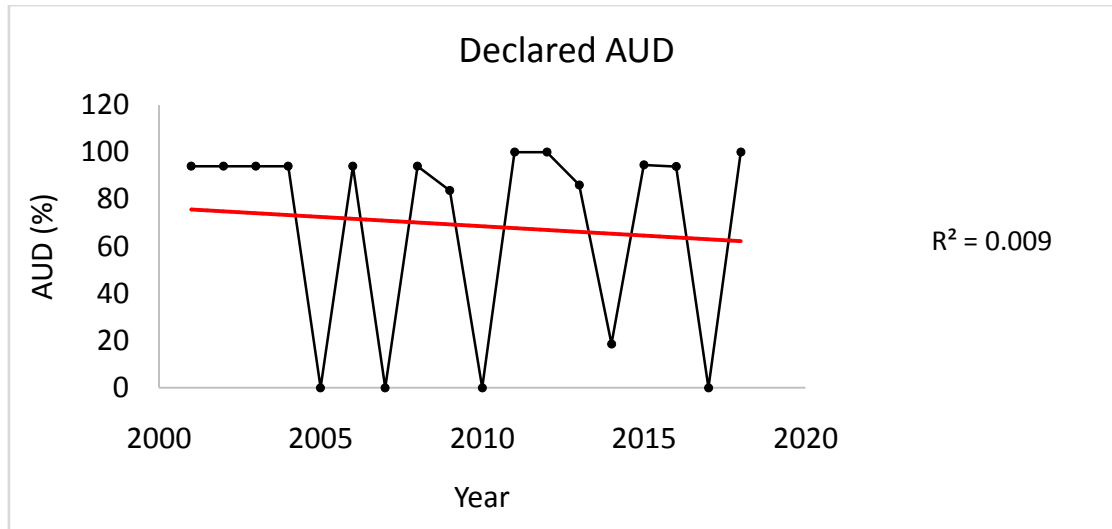
Figure 3. Trend of declared AUD for northern Karnataka
