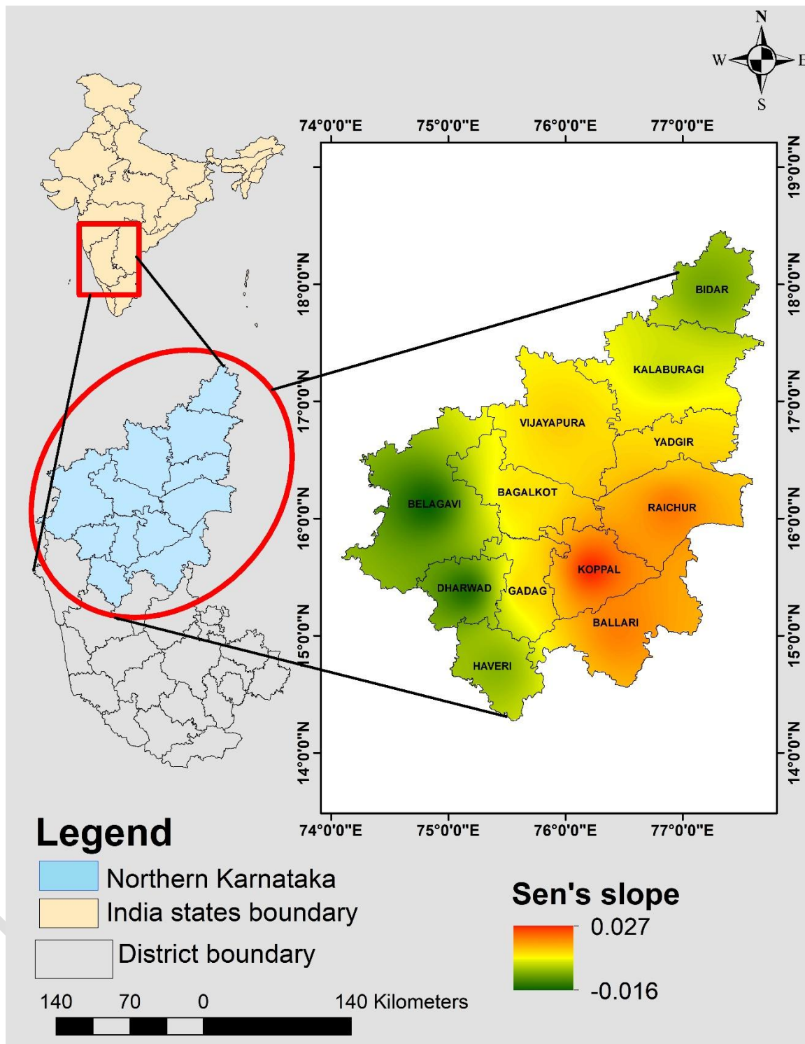
Figure 1. Spatial map of Sen's slope trend magnitude
